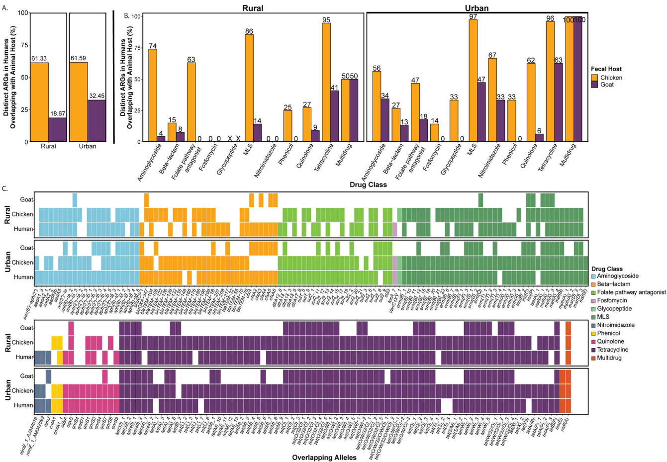
FIG 5 Distinct ARG alleles overlapping between humans and each animal host. (A) Percentage of distinct ARGs identified (using long-read sequencing) in humans that were also found in each animal host. (B) Percentage of distinct ARGs, by drug class, identified (using long-read sequencing) in humans that were also found in each animal host. An “X” indicates that ARGs from that drug class were not detected in humans from that community. (C) ARG alleles overlapping between at least two fecal hosts living in the same community.
