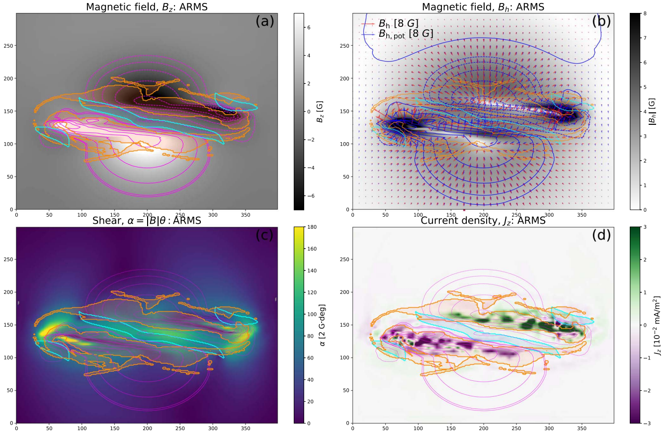
Figure 10. ARMS MHD quantities on the r = R_\odot lower boundary analogous to those presented for an observed X1.6 flare in Figure 4. Panel (a): vertical field B_z . Panel (b): magnitude of the horizontal magnetic field and vector directions of the total and potential components (arrows). Panel (c): distribution of magnetic shear \alpha(x, y) . Panel (d): vertical current density J_z(x, y) . In each panel, the total flare ribbon area during the eruption is denoted as the orange shaded region, while the cyan shaded region indicates the AR PIL. See Section 4.3 for details.
