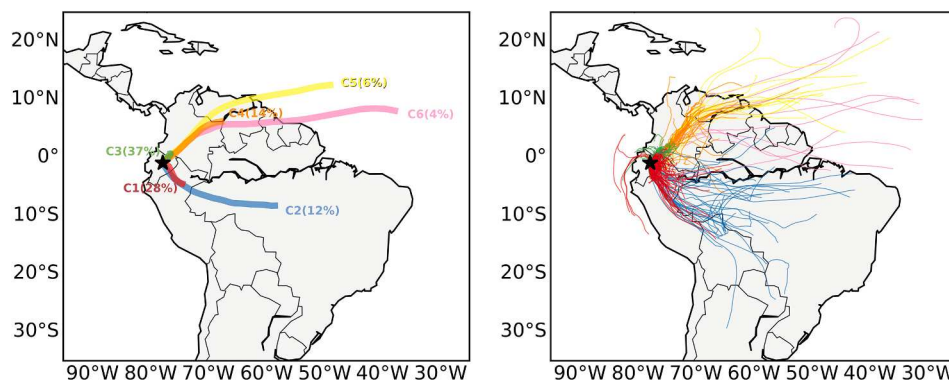
Fig. 9. Seven-day back-trajectories starting at the Ikiam station (star), at 1000 m above ground level ( \sim 730 hPa), from April 2019 to February 2020, considering only back-trajectories starting on precipitation days. The panel on the left shows the average path with the frequency of back-trajectories in percentage for each cluster, and the one on the right shows all back-trajectories.
