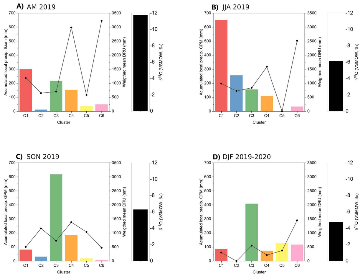
Fig. 10. Precipitation, DRU and \delta^{18}\text{O} associated with each cluster of back-trajectories per season during the monitoring period. Accumulated precipitation (colored bars), weighted mean DRU (line with dots) and weighted mean \delta^{18}\text{O} (black bar) for A) April - May 2019; B) June - July - August 2019; C) September - October - November 2019; and D) December 2019 - January - February 2020.
