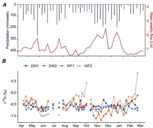
Fig. 8. Weekly hydrograph related to \delta^{18}\text{O} values inside the cave. A) The flow of cave drainage water (red line) with respect to precipitation (blue bars). The cave is recharged directly by rainfall. B) Weekly \delta^{18}\text{O} values of drip water at site 1 (DW1, dark blue dot-line) and at site 2 (DW2, light blue dot-line) and water from river drainages at site 1 (WF1, orange-red dot-line) and at site 2 (WF2, pink dot-line). The figure provides evidence of rapid water entry into the karst system.
