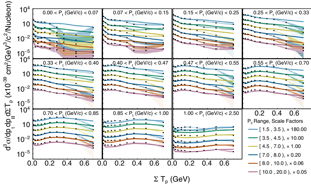
FIG. 1. The flux-averaged triple-differential cross section for quasielastic-like events, d^3\sigma/dp_{||}dp_t d\Sigma T_p , shown as points with colored error bands for designated intervals of p_{||} in panels of p_t . Note the use of scaling factors and log scale to elicit the trends and consistency across all p_{||} . The predictions of the reference model MINERvA tune v4.4.1 are shown as lines in each panel.
