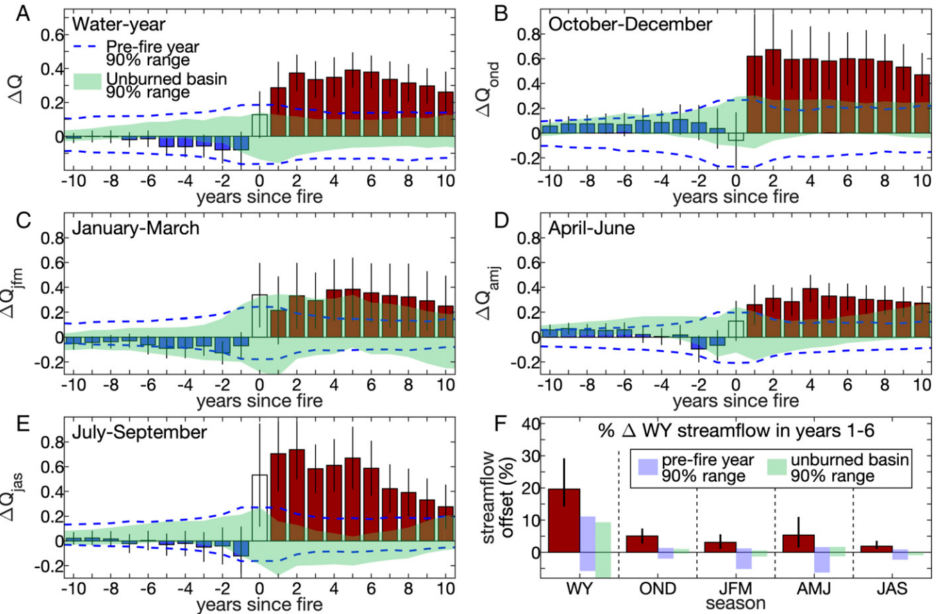
Fig. 3. Multiyear mean water year and seasonal streamflow offsets in heavily burned basins. Streamflow offsets ( \Delta Q ) averaged across only basins where >20\% of forest area burned for (A) the water year and (B–E) the four seasons. Bars indicate multiyear means leading up to (blue) and after (dark red) the fire year (clear). Black vertical lines indicate 90% bounds on means. (F) Dark red bars indicate multibasin median streamflow offset averaged across years 1 to 6 postfire, expressed as percent of estimated total water year (WY) streamflow for the WY and each season: OND, JFM, AMJ, and JAS. Black vertical lines indicate 90% bounds on medians. Blue dashed lines in A–E and blue vertical areas in F bound the inner 90% when each basin's \Delta Q is replaced with 10,000 synthetic time series with prefire variance. Green background in A–E and green vertical areas in F bound the inner 90% of 10,000 repetitions with unburned basins.
