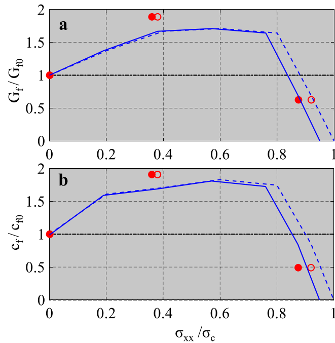
Fig. 2. Gap test results—circle points (empty: as measured on the pad, filled: as inferred for tip vicinity); blue solid curves—calculated based on M7 at plastic pads (dashed) and at tip vicinity. a For mode I fracture energy G_f and b for characteristic size (both normalized by values at zero crack parallel stress).
