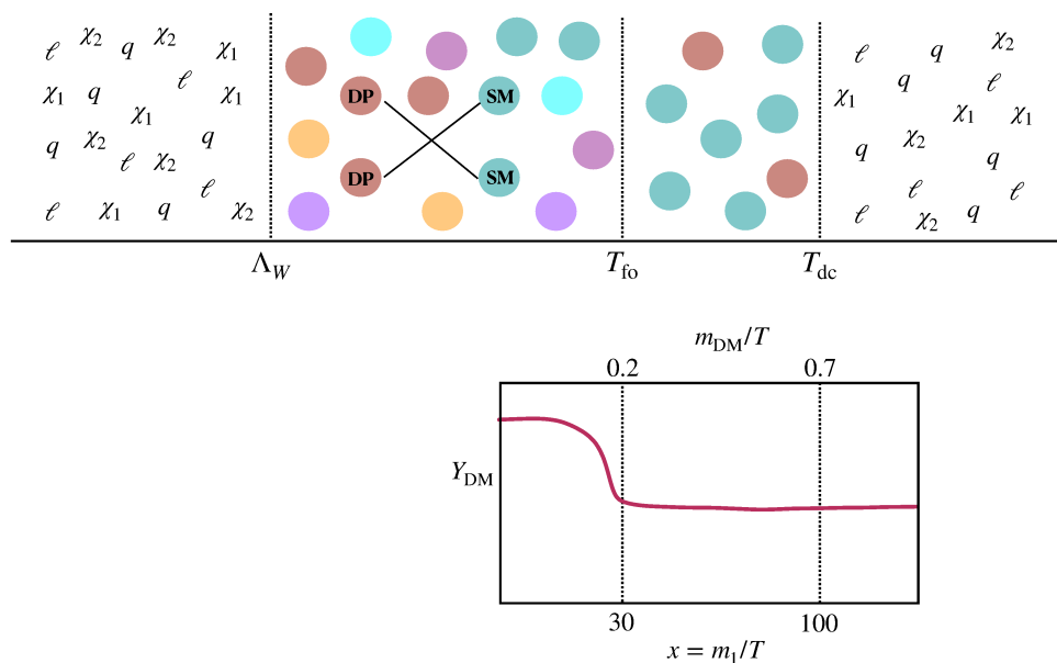
Figure 1. Upper panel: a sketch of the cosmological history of the Universe where we assume a period of weak confinement begins at \Lambda_W , at which point the DM ( \chi_1, \chi_2 ) and SM ( q, \ell ) doublets are bound into weak pions. During this epoch, the freeze-out of dark pions takes place at T_{fo} , followed by deconfinement at T_{dc} . Lower panel: the evolution of the dark pion abundance for a representative value of the freeze-out temperature x_{fo} = m_1/T_{fo} \simeq 30 , corresponding to a temperature of 0.2m_{DM} . In our notation, m_1 and m_{DM} denote the lightest dark pion and the constituent dark matter masses respectively, see section 3 for details.
