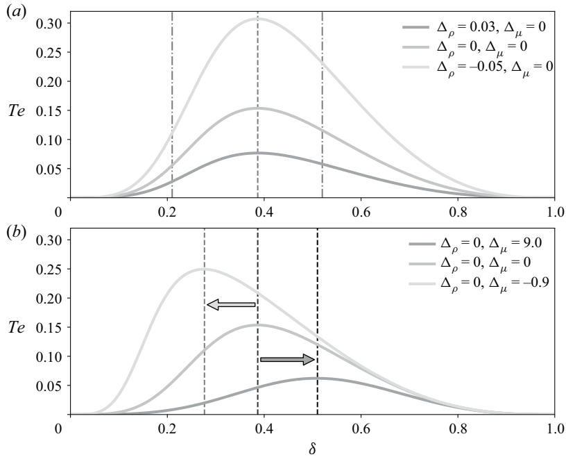
Figure 3. Isolating and comparing the effect of a jump in effective core density to that in effective core viscosity. (a) Upper domain flux function Te for different density jumps \Delta_\rho = 0.03, 0, -0.05 at constant core viscosity \Delta_\mu = 0 . The dashed and dash-dotted lines indicate the flooding point and two inflection points, which are identical for all three scenarios. (b) Upper domain flux function Te for different viscosity jump \Delta_\mu = 9, 0, -0.9 at constant core density. The reference magma density and viscosity contrast are \mathcal{R} = 0.95 and M = 100 . The flooding point position for each case corresponds to the dashed line with the same colour code. The arrows reflect the position shift of the flooding point due to a viscosity jump. Here we only consider the first flux term in (2.20).
