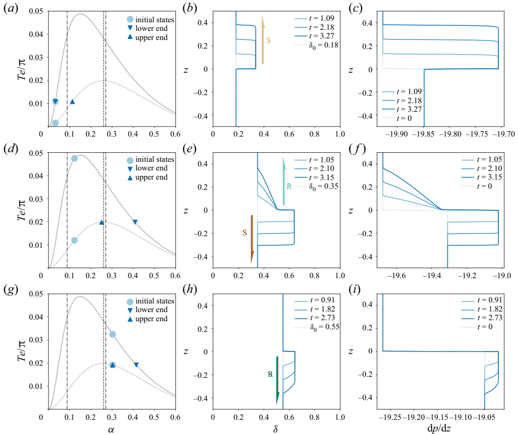
Figure 9. Simulation results for an increase in core viscosity at z=0 and various uniform initial core thicknesses \delta_0 . Panels (a,d,g), (b,e,h) and (c,f,i) represent Te - \alpha diagrams, core thickness evolution and total pressure gradient change. Since the viscosity jump shifts the positions of the flooding and inflection points (see § 3.1), the dashed lines now refer to different flux curves: In panels (a,d,g), the left dash-dotted line and the dashed line refer to the lower flux curve, and the right dash-dotted line refers to the higher flux curve. In all simulations, \mathcal{R} = 0.95 , M = 100 , \Delta_\mu = 9 and \Delta_\rho = 0 .
