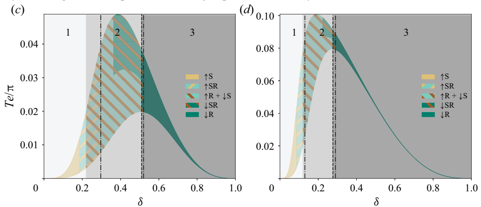
Figure 10. Summary of the dynamic regimes that can arise in response to volatile exsolution. Panels (a,b) are both based on a 5 % decrease in core density, but represent different viscosity contrasts of M = 100 and M = 1000 , respectively. The dashed line and the dash-dotted line indicate the flooding and inflection points. Panels (c,d) are both based on a nine-fold increase in core viscosity. In both cases, \mathcal{R} = 0.95 , \Delta\rho = 0 and \Delta\mu = 9 , but the initial viscosity contrast is M = 100 in panel (c) and M = 10^4 in panel (d). The dashed line and the dash-dotted line on the left indicate the flooding and left inflection points of the lower flux function, while the dash-dotted line on the right represents the right inflection point of the higher flux function. Regions in panels (b,c) with dark cyan sitting above light cyan indicate the existence of both ascending and descending rarefactions.
