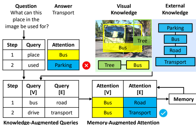
Figure 1. Based on neural module networks and explicit knowledge representation, we develop knowledge-augmented queries and memory-augmented attention to jointly reason about both the visual [V] and external [E] knowledge. These query and attention augmentation methods generalize explainable visual reasoning models to better answer knowledge-requiring questions.
