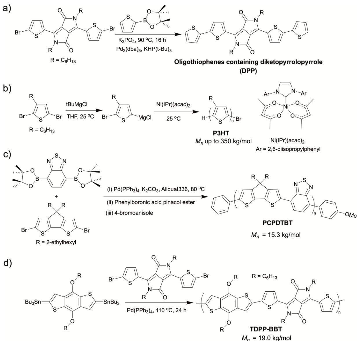
Scheme 1 a) Synthesis of diketopyrrolopyrrole (DPP) containing oligothiophenes via Suzuki coupling. 12 b) Synthesis of P3HT via Kumada catalyst transfer polycondensation (KCTP). 13 c) Synthesis of poly[4,4-bis(2-ethylhexyl)-4Hcyclopenta[2,1-b;3,4-b']dithiophene-2,6-diyl-alt-2,1,3-benzothiadiazole-4,7-diyl] (PCPDTBT) via Suzuki coupling. 14 d) Synthesis of DPP containing copolymers (TDPP-BBT) via Stille coupling. 15
