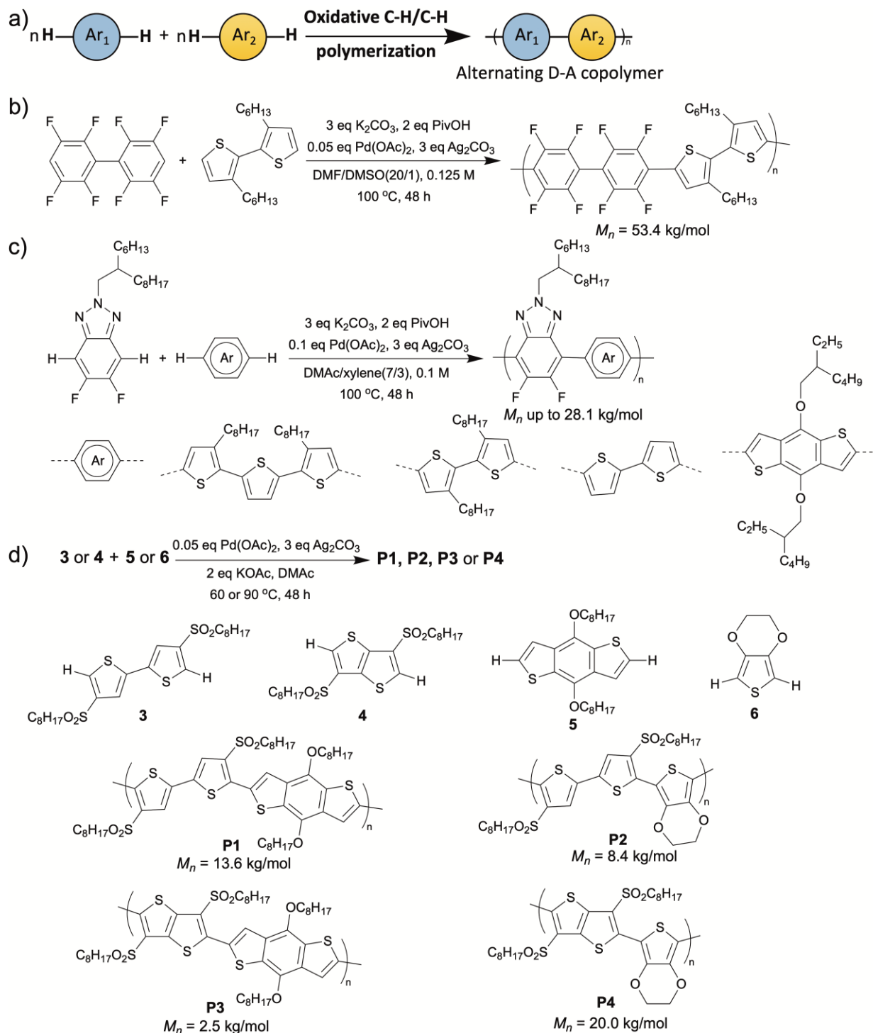
Scheme 8 a) A general synthetic scheme of D-A semiconducting copolymers via CDC. b) Palladium/silver catalyzed CDC polymerization. c) Synthesis of fluorinated benzotriazole containing D-A conjugated copolymers via CDC. d) The CDC polymerizations of various D-A conjugated copolymers.
