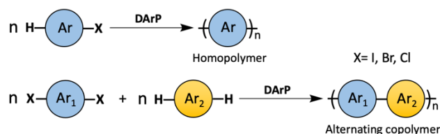
Scheme 4 A general scheme of DAP to synthesize semiconducting homopolymer and alternating copolymer.
