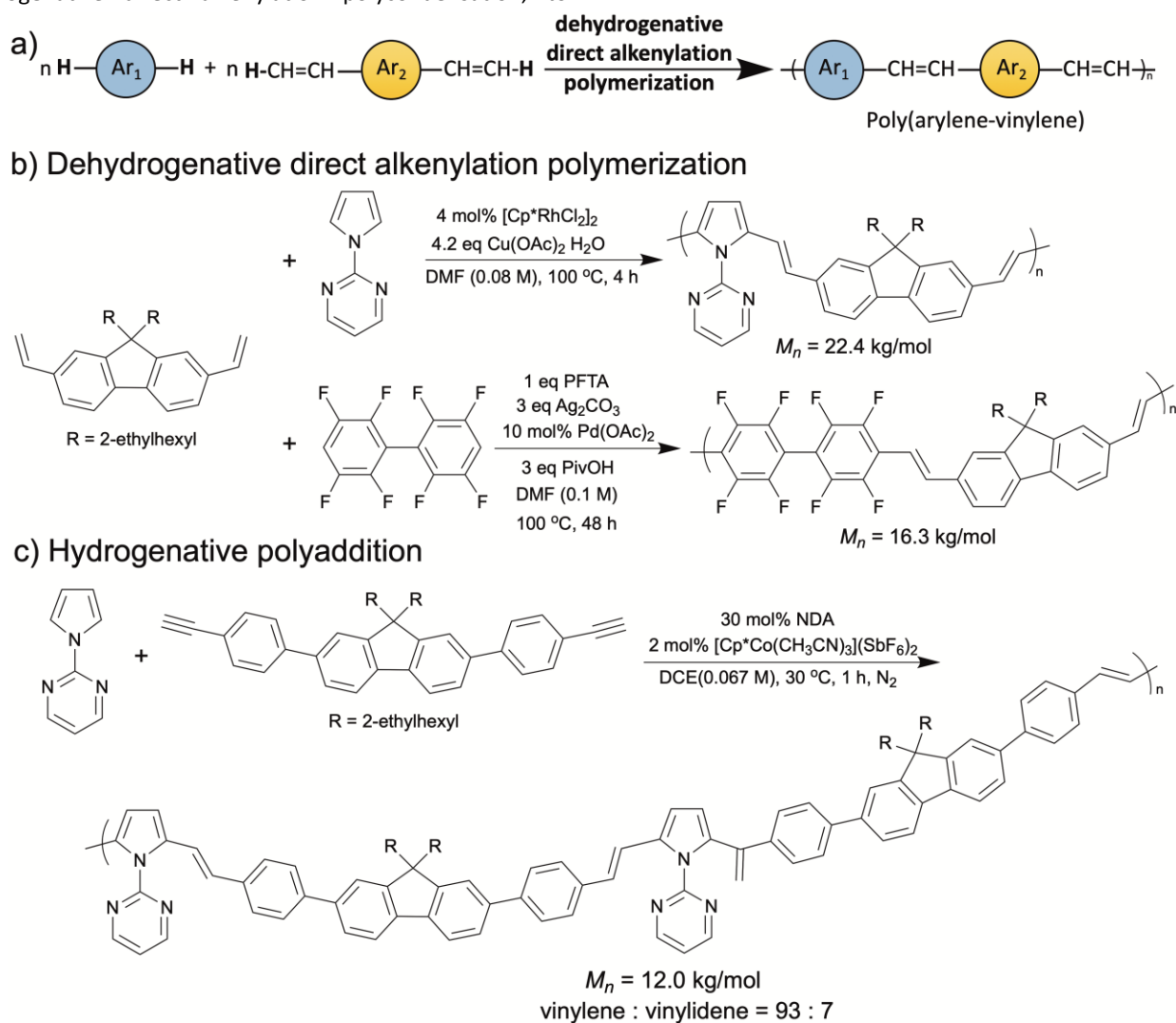
Scheme 9 a) A general scheme of dehydrogenative direct alkenylation polymerization to synthesize poly(arylene-vinylene)s. b) Rhodium- and palladium catalyzed dehydrogenative direct alkenylation polymerizations to synthesize poly(arylene-vinylene)s. c) Cobalt-catalyzed hydrogenative polyaddition to synthesize poly(arylene-vinylene)s.
