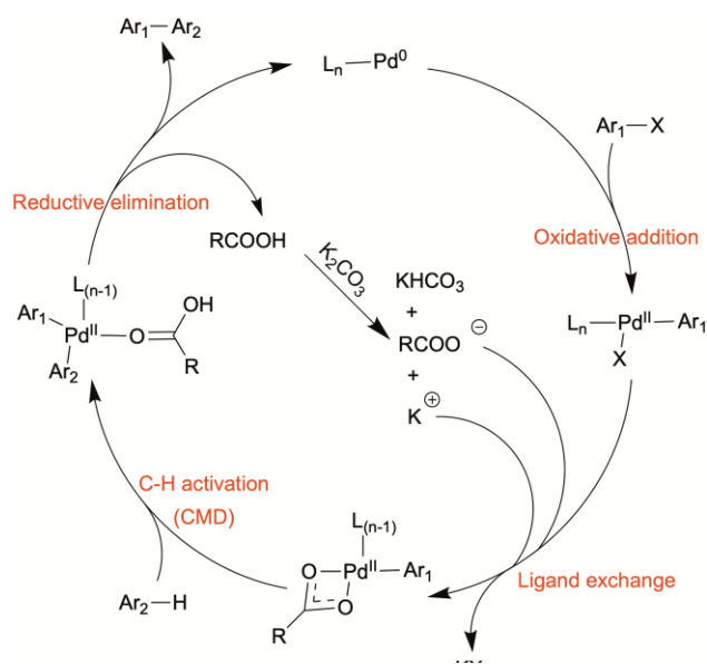
Scheme 3 A plausible catalytic cycle of direct arylation.
