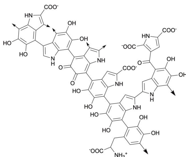
Scheme 14 Part of chemical structure of two-dimensional melanin sheet (arrows means the positions where the sheet could extend from).
