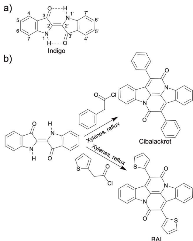
Scheme 13 a) Chemical structure of indigo. b) Annulation reaction of indigo to synthesize cibalackrot and BAI.
