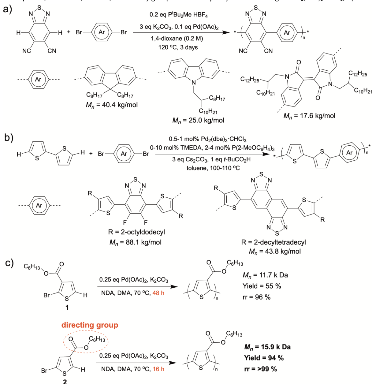
Scheme 5 a) Synthesis of DCBT containing conjugated D-A copolymers via DARp. b) Synthesis of unsubstituted bithiophene containing D-A copolymers via DARp using a mixed ligand catalyst to suppress branching side reactions. c) Synthesis of highly regioregular P3HET via DARp with the ester functionality as the directing group to promote regioregularity.
