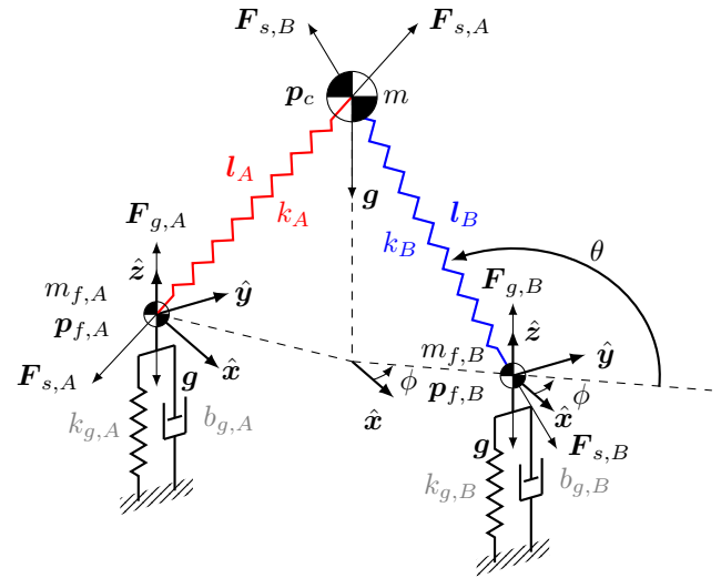
Fig. 1: The extended 3D Dual Spring-Loaded Inverted Pendulum (Dual-SLIP) model in compliant terrain during double support (DS) at Touchdown.
