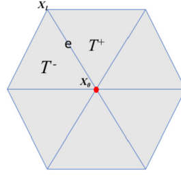
Fig. 2. A macroelement M \in \mathcal{M}_h associated to an interior node x_0 in the mesh \mathcal{T}_h .
