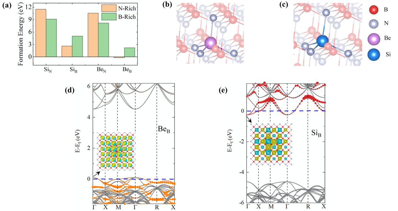
FIG. 1. Doping cBN: (a) Formation energies for intentional shallow dopants (Be and Si) in N-rich and B-rich conditions. Substitutional defect, (b) Be B for p doping cBN, and (c) Si B , for n doping cBN. Fat band (projected band structure) plots showing atomic contributions of (d) Be and (e) Si to the band structure of doped cBN represented by orange- and red-colored dots, respectively. The dot size is proportional to the contribution of the dopant states in the corresponding Bloch wave function. The zero of the energy is set at the Fermi energy ( E_F ). The inset in (d) is the charge density plot of the state (at the \Gamma point) introduced just above the Fermi level. The inset in (e) shows the state (at the \Gamma point) introduced just below the Fermi level, with contributions from nearly all atoms, including Si. Yellow (blue) colors in the charge density plots correspond to positive (negative) isovalues of the plotted quantity, [\text{sign}(\psi) \times |\psi|^2] , where \psi is the selected wave function at the \Gamma point.
