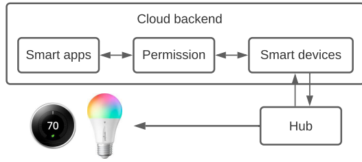
Fig. 1: The architecture of SmartThings IoT platform.
