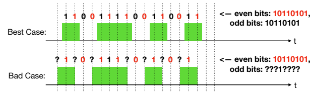
Figure 3: Timing diagram of a decoder searching for tag ID 0b10110101 in two possible cases. Dotted vertical lines are when a camera samples a frame. A green box means a tag is in an “on” state. The top is the best/typical case, where the camera is out of phase with the tag. The bottom shows a bad case where the camera’s frame capture is perfectly in sync with a tag’s blinking and some values are unknown to the decoder. Since our system matches using even or odd video frames, the unknown values do not affect the decoder’s ability to find a tag ID.
