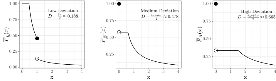
Figure EC.2 Tight distributions for Theorem 2
