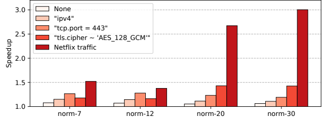
Figure 12: Speedup from Compiled Filter Code —Native code generation can result in 5.4%–300.4% speedups over runtime filter interpretation, depending on filter complexity and the offered traffic. “Netflix traffic” refers to a 32 predicate filter for known Netflix domains and IP prefixes used by Bronzino et al. [16] to collect Netflix traffic features.
