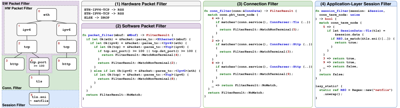
Figure 3: Filter Decomposition and Code Generation —We show how the filter ( ipv4 and tcp.port>=100 and tls.sni~'netflix' ) or http is decomposed and executed. Retina parses the specified filter expression into a predicate trie representation, and generates (1) a set of NIC-compatible flow rules, (2) a more expressive packet filter, (3) a connection filter, and (4) an application-layer session filter. Flow rules are installed on the NIC, while the software filter functions are compiled and inlined at their respective processing layers. Native code generation can result in up to 3× higher throughput over runtime interpretation, depending on the filter and traffic (Appendix B). Note: we truncate full path names and other expansions for readability.
