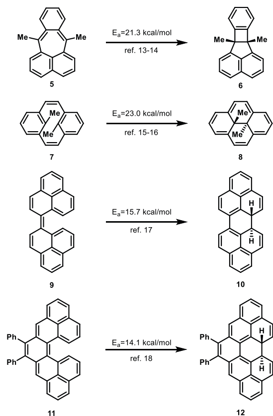
Figure 2. Experimental activation energies for energetically preferred, symmetry-forbidden electrocyclizations.
