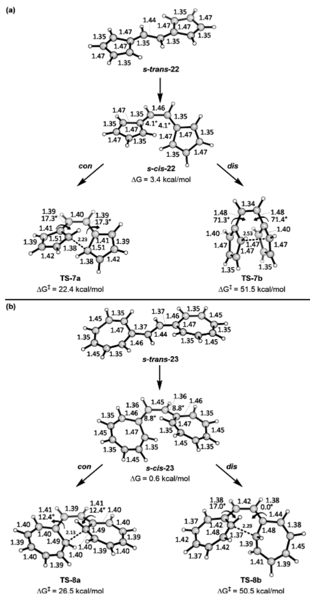
Figure 9. Bond lengths and torsion angles of (a) vinylogous pentafulvalene and (b) vinylogous heptafulvalene along with transition states for their electrocyclizations. All are closed-shell wave functions.
