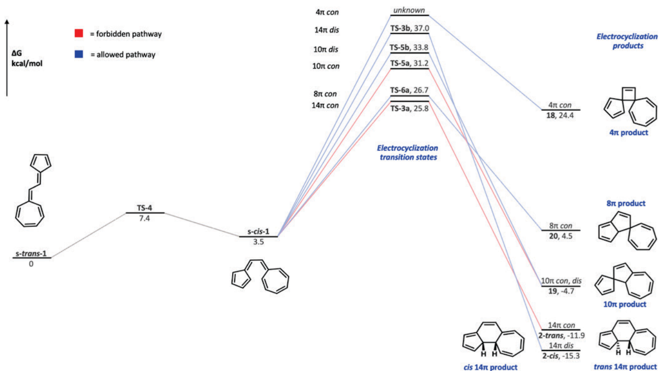
Figure 6. Free energy diagram for electrocyclicization of s-cis -1 via 4, 8, 10, and 14 conrotatory and disrotatory pathways. All structures have closed-shell wave functions except for TS-5a.
