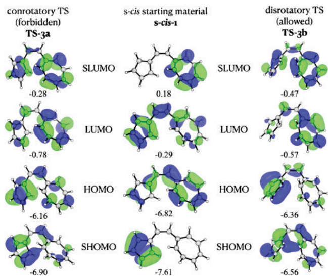
Figure 13. Two highest occupied and two lowest vacant orbitals of vinylogous sesquifulvalene in the s-cis conformation and in the 14 con and dis transition states.
