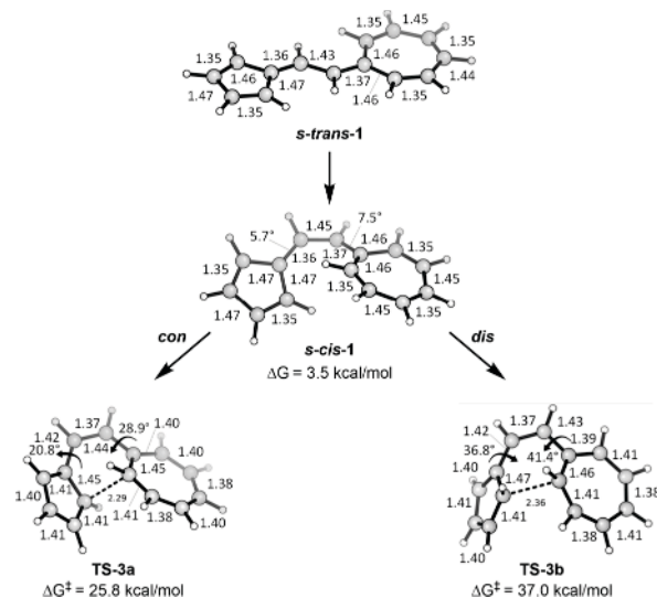
Figure 5. Geometries of s-trans and s-cis reactants and transition state geometries for conrotatory and disrotatory 14 electrocyclicizations.
