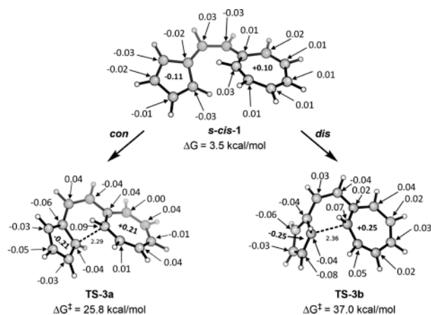
Figure 12. Charges in s-cis vinylogous sesquifulvalene and the forbidden and allowed 14 transition states.
