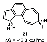
Figure 8. Final product formed by thermolysis of 2- trans .
