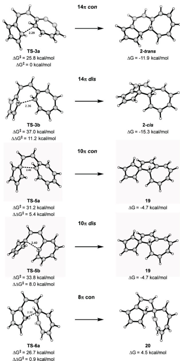
Figure 7. Transition states of 14-, 10-, and 8-electron electrocyclizations of s-cis -1.
