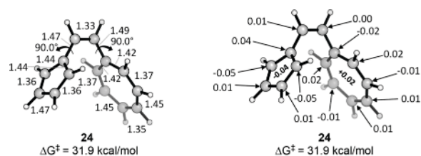
Figure 10. Diradical structure formed from the vinylogous sesquifulvalene by rotating both rings to 90° relative to the connecting ethylene moiety. Geometries and Hirshfeld charges (Hs summed into Cs) are shown.
