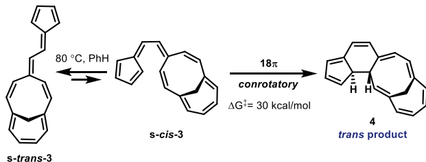
Figure 1. Symmetry-forbidden conrotatory electrocyclizations of (a) 14 vinylous sesquifulvalene and (b) the related 18 fulvene hendecafulvene system reported by Prinzbach. Reactions were performed in benzene. Energetics were measure by Prinzbach. 1,2
