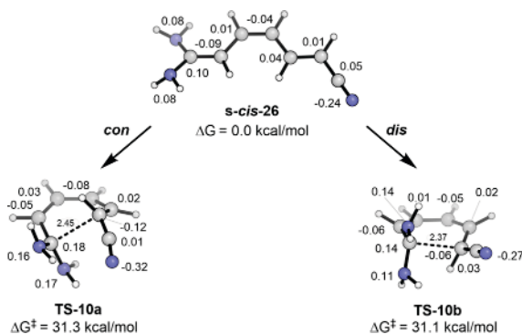
Figure 16. Forbidden conrotatory and allowed disrotatory transition states for electrocyclicization of cis,trans -1,1-diamino-6-cyanohexatriene. Hirshfeld charges are shown by each atom.
