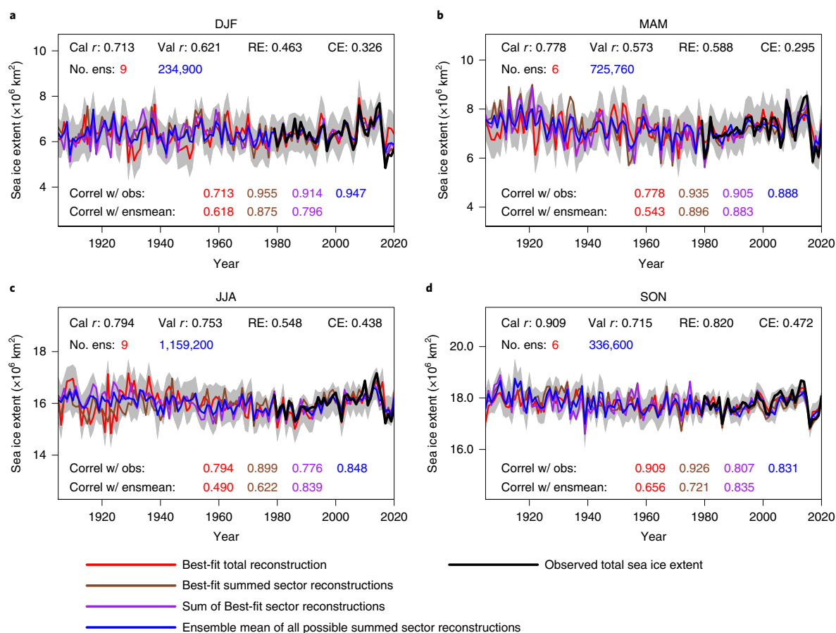
Fig. 2 | Seasonal Antarctic total sea ice extent comparisons, 1905–2020. a–d , Various ways of representing the total seasonal Antarctic sea ice extent reconstruction, along with various reconstruction skill metrics for the best-fit reconstruction (red lines). Cal r , calibration correlation; val r , validation correlation; RE, reduction of error; CE, coefficient of efficiency. The best-fit reconstruction (red lines) is the highest-performing ensemble member calibrated specifically to the observed total sea ice extent. The best-fit summed sector reconstruction (brown lines) is the ensemble member from all possible sums of the individual sector ensemble members, while the ensemble mean (blue lines) is the average of all these possible sector reconstruction sums. The sum of the best-fit sector reconstructions (purple lines) is the sum of the highest-performing sector reconstruction ensemble members that have been specifically calibrated to the observed sector sea ice extent. The correlation of all reconstructions with the observations (correl w/ obs) and the correlation of the reconstructions with the ensemble mean (correl w/ ensmean) are given at the bottom of each plot, with the colours representing the various reconstructions labelled in the legend below the figure. The number of ensemble members (no. ens) is also given for the best-fit reconstruction (red) as well as for the ensemble mean (blue). The grey shading is as in Fig. 1 and approximates the reconstruction uncertainty as the greater of 1.96 times the standard deviation of the ensemble members or 1.96 times the standard deviation of the best-fit reconstruction ensemble member.
