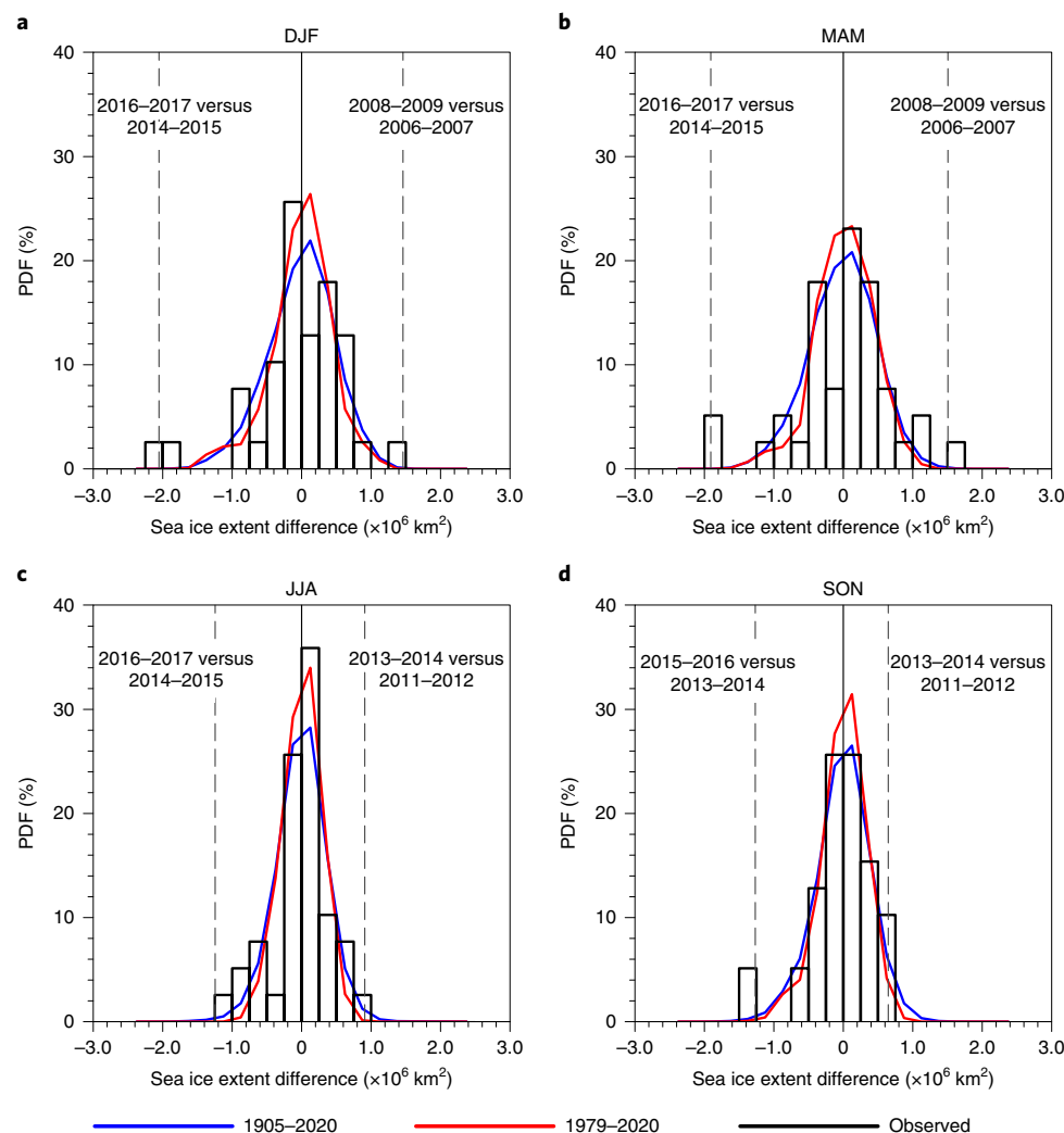
Fig. 5 | Changes in 2-year average seasonal sea ice extent. a–d , Seasonal probability density functions (PDFs, in %) for differences (following years minus preceding years) in consecutive, non-overlapping 2-year mean Antarctic total sea ice extent from observations (black, plotted as a bar chart) and in all Antarctic total sea ice extent reconstruction ensemble members from 1979 to 2020 (red) and 1905 to 2020 (blue). The dashed vertical lines indicate the minimum and maximum differences in the observations, with the 2-year mean periods corresponding to these record differences given in the upper corners of each panel.
