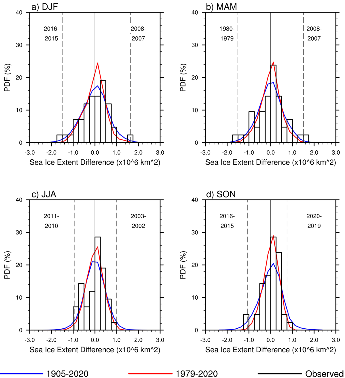
Extended Data Fig. 3 | Changes in year-to-year seasonal sea ice extent. Seasonal probability density functions (PDF, in %) for differences (following year minus preceding year) in consecutive one year values in observed Antarctic total sea ice extent (black, plotted as a bar chart) and in all Antarctic total sea ice extent ensemble members from 1979-2020 (red) and 1905-2020 (blue). The dashed vertical lines indicate the minimum and maximum differences in observations, with the years corresponding to these record differences given in the upper corners within each panel.
