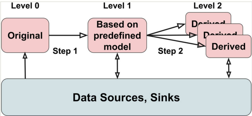
Figure 1. Generalized flow of data in ecological synthesis. Level 0 (L0) are incoming, original data, ideally, already archived in the repository with complete metadata and contributed by those close to the research. Level 1 (L1) data packages (also in the repository) are formatted according to a predefined model, in this case, ecocomDP. Researchers are able to use L1 as inputs with its code to speed their analyses and generate Level 2 (L2) data. An archive of the L2 data package in the same repository is recommended. Data sources and sinks may be a repository (e.g., EDI) another data provider (e.g., NEON) or aggregator (e.g., GBIF). Reproduced from O'Brien et al. (2021).
