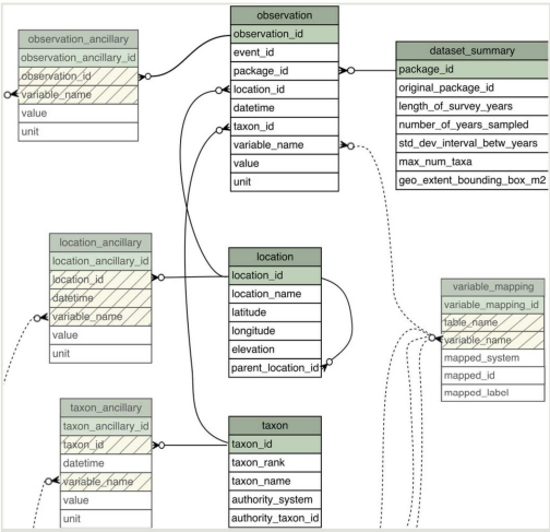
Figure 2. The ecocomDP model shown with relational database notation for foreign keys and relationships (e.g, lines ending in crow's-foot indicate 1:many relationships). Semi-transparent tables are optional. Medium green fields in each table are the primary key. Yellow/hashed fields are a combined unique constraint. IDs (suffixed, "_id"), must be unique within a table, as in an relational database. Full documentation can be found here . Reproduced from O'Brien et al. (2021).
