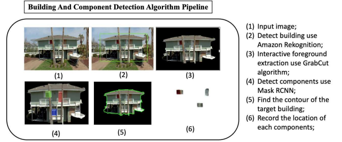
Fig. 7. Building and component detection algorithm pipeline
