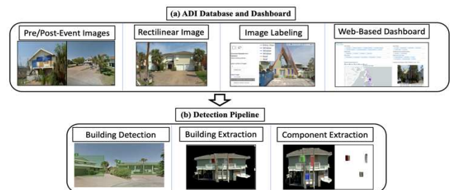
Fig. 1. System workflow.
