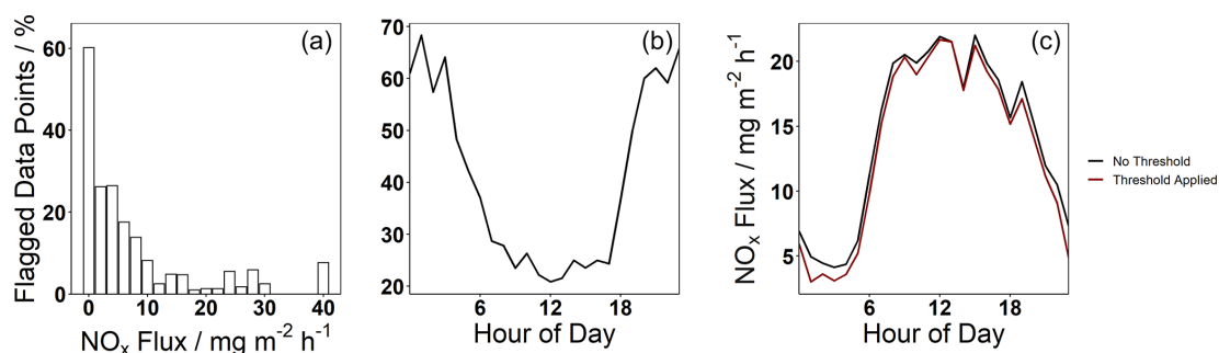
Figure 4. (a) Percentage of flux records flagged by quality control routines in 2 \text{ mg m}^{-2} \text{h}^{-1} bins. (b) Percentage of flux records flagged by quality control routines by hour of day. (c) \text{NO}_x flux diurnal cycle; black has had all records flagged by quality control routines removed, and red has only had them removed if the flux magnitude was also greater than 5 \text{ mg m}^{-2} \text{h}^{-1} .
