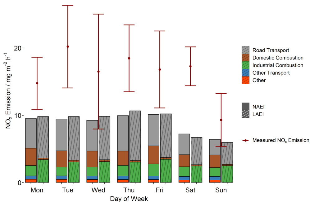
Figure 10. Daily averaged measured \text{NO}_x emissions by day of week shown as red points and stacked bars of simulated emissions coloured by source sector for the NAEI (solid colour) and LAEI (hatched).
