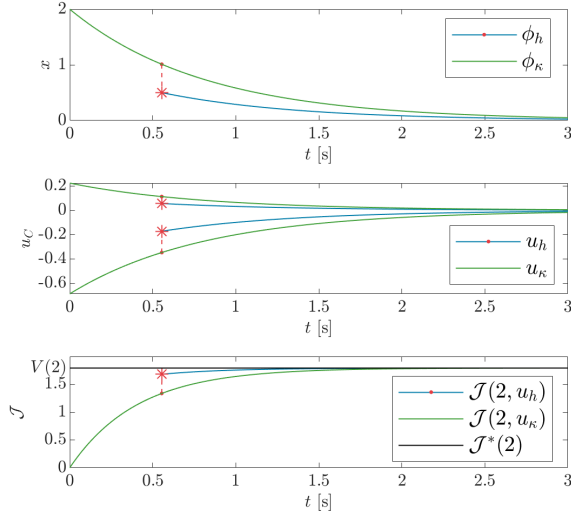
Figure 1: Nonunique solutions attaining minmax optimal cost for a = -1, b_1 = b_2 = 1, \delta = \xi = 2, \mu = 1, \sigma = 0.5, Q_C = 1, R_{C1} = 1.304, R_{C2} = -4 , and P = 0.4481 . Continuous solution (green). Hybrid solution (blue and red).
