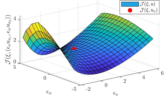
Figure 3: Saddle point behavior in the cost of solutions to bouncing ball from \xi = (1, 1) when varying the feedback gains around the optimal value. The cost is evaluated on solutions (\phi, u) \in \mathcal{S}_{\mathcal{H}}^{\infty}(\xi) with feedback law variations specified by \epsilon_u and \epsilon_w in u = (\epsilon_u \kappa_1(\phi), \epsilon_w \kappa_2(\phi)) .
