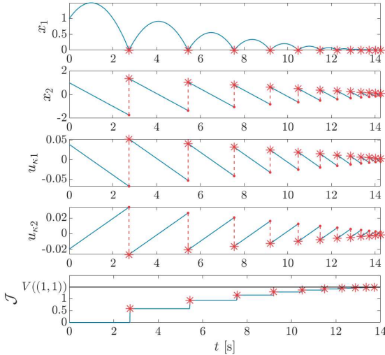
Figure 2: Bouncing ball solutions attaining minimum cost under worst-case u_2 , with \lambda = 0.8 , R_{D1} = 10 , R_{D2} = -20 , and Q_D = 0.189 .
