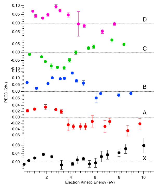
Fig. 5. Mean PECD ( 2\widehat{b}_1 , see text) versus electron kinetic energy given for the \Delta - \text{Ru}(\text{acac})_3 enantiomer, for the first five experimental bands described in the text (see Figs. 3 and 4, and Table 2). Note that the \Lambda enantiomer data have been negated and are also included in these plots. The error bars reflect statistical errors (see Figure 4's caption) except those corresponding to photon energies where both enantiomers were studied (8, 11, 12 and 15 eV), which also contain systematic errors accounting for the observed deviations from a perfect mirror behaviour.
