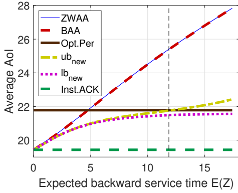
Fig. 2. (lb_{new}, ub_{new}) versus existing results — log-normal \mathbb{P}_Y
