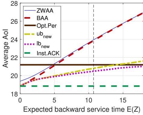
Fig. 3. (lb_{new}, ub_{new}) versus existing results — composite log-normal \mathbb{P}_Y .
