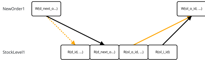
Figure 3: Another potential isolation bug reported by IsoBugView.
