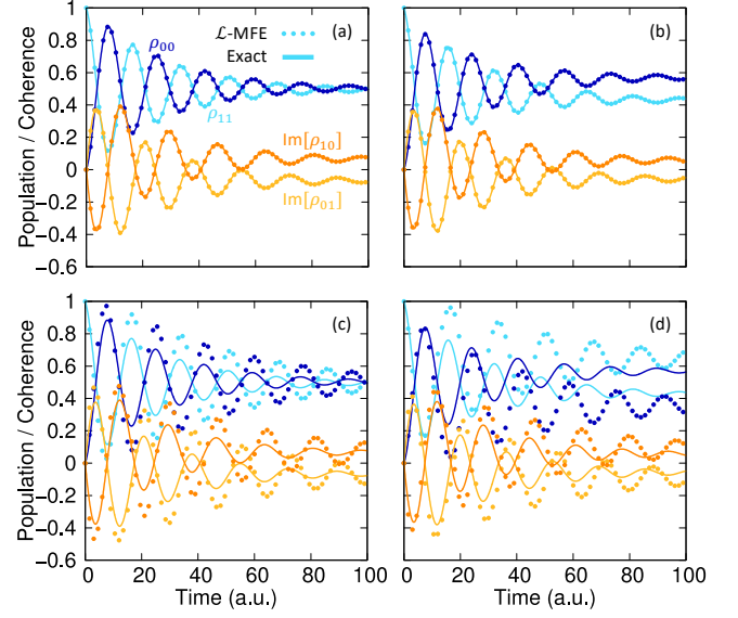
FIG. 2. Dynamics of (a) Model 3 and (b) Model 4. The solid lines are exact Lindblad dynamics while the dotted lines are the \mathcal{L} -MFE method. The cyan lines are the population of state |1\rangle , the dark blue lines are the population of state |0\rangle , the darker orange lines represent \text{Im}[\rho_{10}] , and the lighter orange lines represent \text{Im}[\rho_{01}] . Panels (c)-(d) present the same calculation as (a) and (b), but without any random phase (by setting \theta_\xi = 0 in Eq. 69b) in the \mathcal{L} -MFE method.
