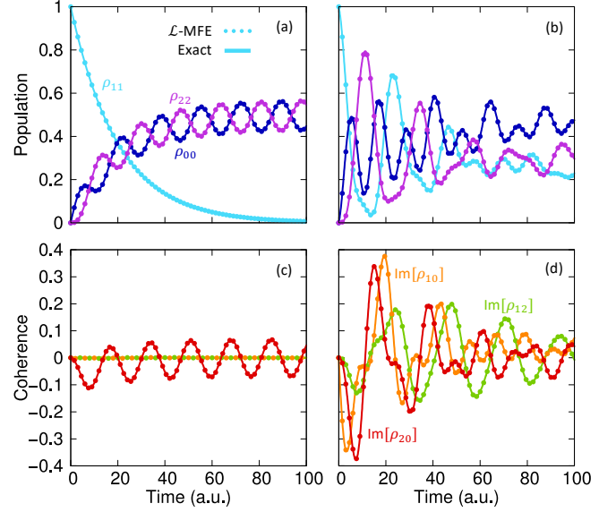
FIG. 4. Dynamics of Models 5 (a,c) and Model 6 (b,d). The solid lines are exact Lindblad dynamics while the dotted lines are the \mathcal{L} -MFE method. Panels (a) and (b) present the diagonal populations, with \rho_{00}(t) (dark blue), \rho_{11}(t) (cyan), and \rho_{22}(t) (magenta). Panels (c) and (d) present the off-diagonal coherences, with \text{Im}[\rho_{10}](t) (orange), \text{Im}[\rho_{12}](t) (green), and \text{Im}[\rho_{20}](t) (red).
