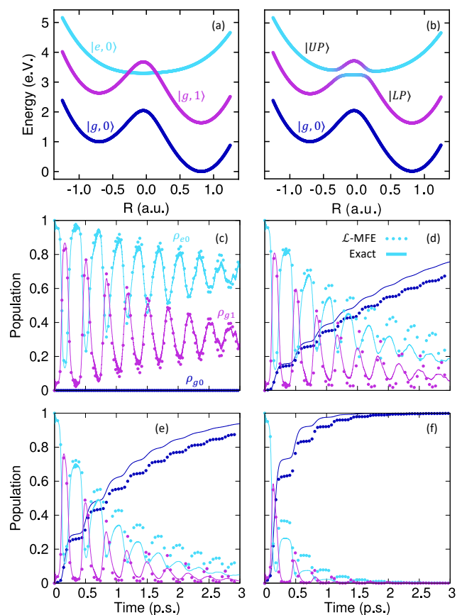
FIG. 7. Potential energy surfaces (PESs) and population dynamics of the model isomerization reaction coupled to the cavity. Panel (a) presents the diabatic PESs where the dark blue line is the |g, 0\rangle PES, the cyan line is the |e, 0\rangle PES, and the magenta line is the |g, 1\rangle PES. Panel (b) presents the adiabatic PESs where the dark blue line is the ground state |g, 0\rangle PES, the middle line (labeled |LP\rangle ) is the lower polariton PES, and the upper line (labeled |UP\rangle ) is the upper polariton PES. The colors along the adiabatic PESs represent the diabatic character at each nuclear position. Panels (c)-(f) present the population dynamics where (c) uses a decay rate of \Gamma = 0 , (d) uses \Gamma = 1 meV, (e) uses \Gamma = 2 meV, and (f) uses \Gamma = 8 meV. The solid lines are exact Lindblad dynamics while the dotted lines are the \mathcal{L} -MFE method. The dark blue lines are the state |g, 0\rangle populations, the cyan lines are the state |e, 0\rangle populations, and the magenta lines are the state |g, 1\rangle populations.
