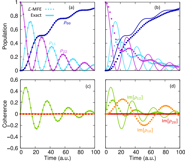
FIG. 5. Dynamics of Model 7 using (a,c) the \mathcal{L} -MFE approach and (b,d) a modified \mathcal{L} -MFE approach with the random phase only applied to state |1\rangle . The solid lines are exact Lindblad dynamics while the dotted lines are the original or modified \mathcal{L} -MFE approach. Panels (a) and (b) present the diagonal populations, with \rho_{00}(t) (dark blue), \rho_{11}(t) (cyan), and \rho_{22}(t) (magenta). Panels (c) and (d) present the off-diagonal coherences, with \text{Im}[\rho_{10}](t) (orange), \text{Im}[\rho_{12}](t) (green), and \text{Im}[\rho_{20}](t) (red).
