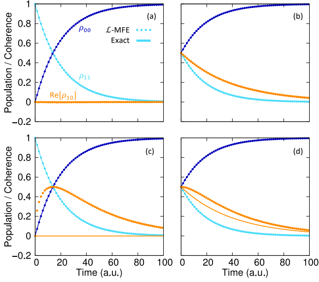
FIG. 1. Dynamics of (a) Model 1 and (b) Model 2. The solid lines are exact Lindblad dynamics while the dotted lines are the \mathcal{L} -MFE method. The cyan lines are the population of state |1\rangle , the dark blue lines are the population of state |0\rangle , and the orange lines represent \text{Re}[\rho_{10}] . Panels (c)-(d) present the same calculation as (a) and (b), but without any random phase (by setting \theta_\xi = 0 in Eq. 69b) in the \mathcal{L} -MFE method, thus generating artificially large coherence.
