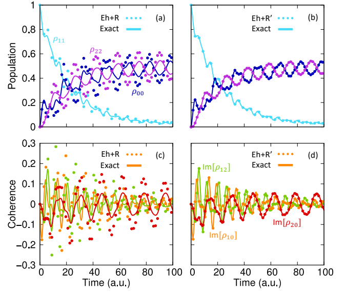
FIG. 6. Dynamics of Model 8 using (a,c) the original Ehrenfest+R approach (labeled as Eh+R) and (b,d) the Ehrenfest+R approach using the modified \gamma'_R from Eq. 75 (labeled as Eh+R'). The modified Ehrenfest+R dynamics (Eh+R') are identical to those obtained from the \mathcal{L} -MFE method for this model. The solid lines are exact Lindblad dynamics while the dotted lines are the original or modified Ehrenfest+R approach. Panels (a) and (b) present the diagonal populations, with \rho_{00}(t) (dark blue), \rho_{11}(t) (cyan), and \rho_{22}(t) (magenta). Panels (c) and (d) present the off-diagonal coherences, with \text{Im}[\rho_{10}](t) (orange), \text{Im}[\rho_{12}](t) (yellow), and \text{Im}[\rho_{20}](t) (red).
