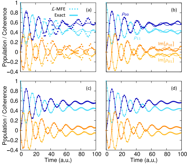
FIG. 3. Dynamics of Model 4 with different numbers of trajectories. The solid lines are exact Lindblad dynamics while the dotted lines are the \mathcal{L} -MFE method. The numbers of trajectories used are (a) 10, (b) 100, (c) 1,000, and (d) 10,000.
