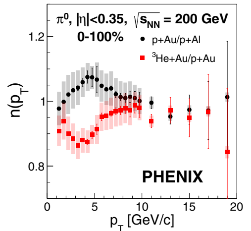
FIG. 8. Exponent according to Eq. (5) as a function of transverse momenta extracted from p + \text{Au}/p + \text{Al} and ^3\text{He} + \text{Au}/p + \text{Au} collision systems. The uncertainties from the N_{\text{coll}} calculations and from the overall normalization of p + p cancel in these ratios.
