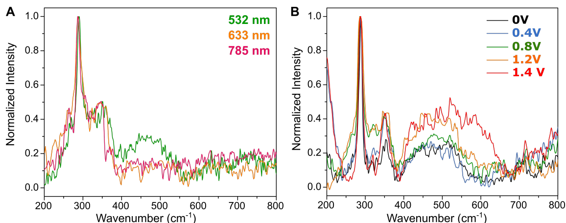
Figure 4. Raman Characterization of the OER Catalytic Mechanism of the Hybrid Plasmonic Photocatalyst. (A) Raman spectra of L-NR-NCs drop-casted thin film at different excitation wavelengths of 532 nm (green), 633 nm (orange) and 785 nm (red). (B) Raman spectra of L-NR-NCs drop-casted thin film on ITO substrate with different applied bias in the range of 0 - 1.4 V. All spectra were collected with 532 nm excitation.
