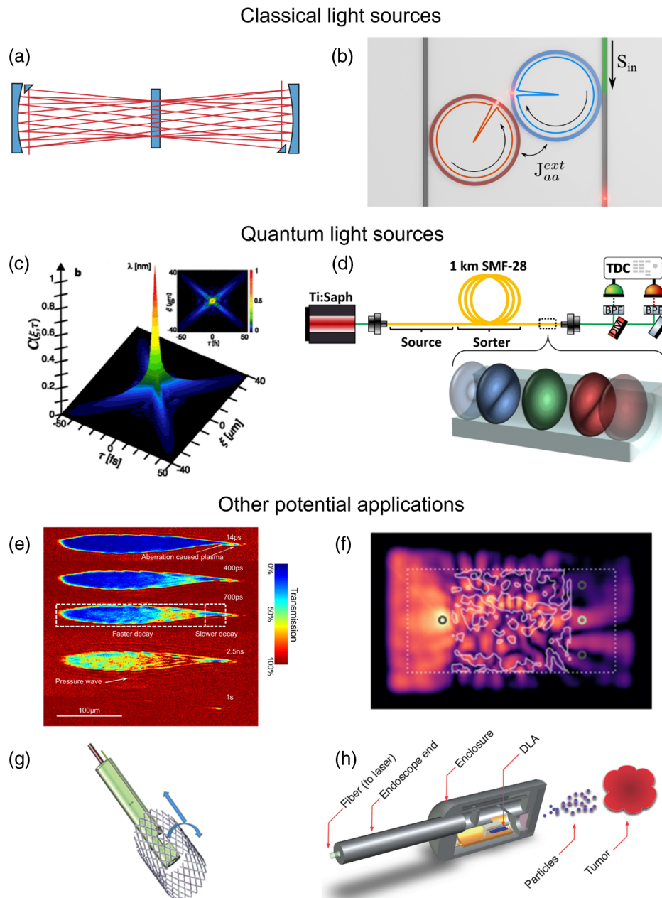
Fig. 4. Platforms and potential applications of multimode nonlinear photonics. (a) Multipass cells [234] and (b) integrated photonic structures [235] are flexible platforms wherein nonlinear multimode waves may be controlled to produce new forms of multimode coherent light. Spatiotemporal and multimode considerations are necessary to describe many spontaneous nonlinear processes for generating non-classical light, e.g., (c) in bulk media [92], or to engineer (d) fiber-based [236] or integrated [93] sources of non-classical multimode light. Applications that may benefit from coherent multimode light include the (e) intrinsically spatiotemporal interactions in laser materials processing and laser-plasma interactions [100]. Multimode nonlinear optical dynamics can be used for information processing, such as all-optical phase-retrieval [237], or (f) machine learning inference [115,238]. (g) Photoacoustic [239] and other biomedical optical imaging modalities, as well as (h) integrated laser-driven particle accelerators [110], may benefit from multimode fiber endoscope-based deployment [240–244]. Figures adapted from [92,100,110,234–236,238,245] with permission.
