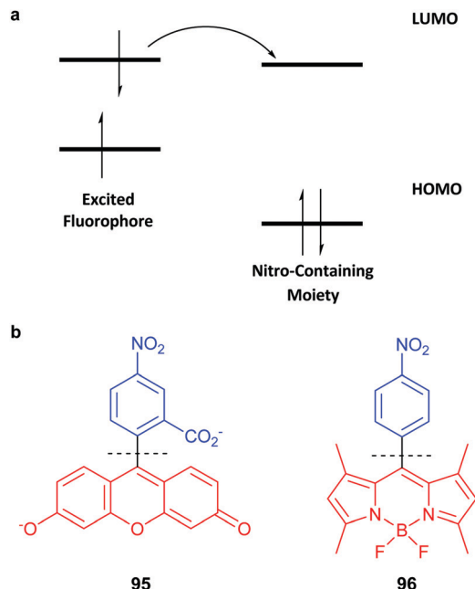
Fig. 31 (a) The mechanism of donor-excited photoinduced electron transfer (d-PET). (b) Examples of chromophores in which electron-accepting and electron-donating parts are electronically disconnected.
