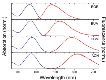
Fig. 3 Absorption (blue) and emission (red) spectra of compound 9 in solvents of different polarity. Reprinted with permission from ref. 69 Copyright 2012 American Chemical Society.
