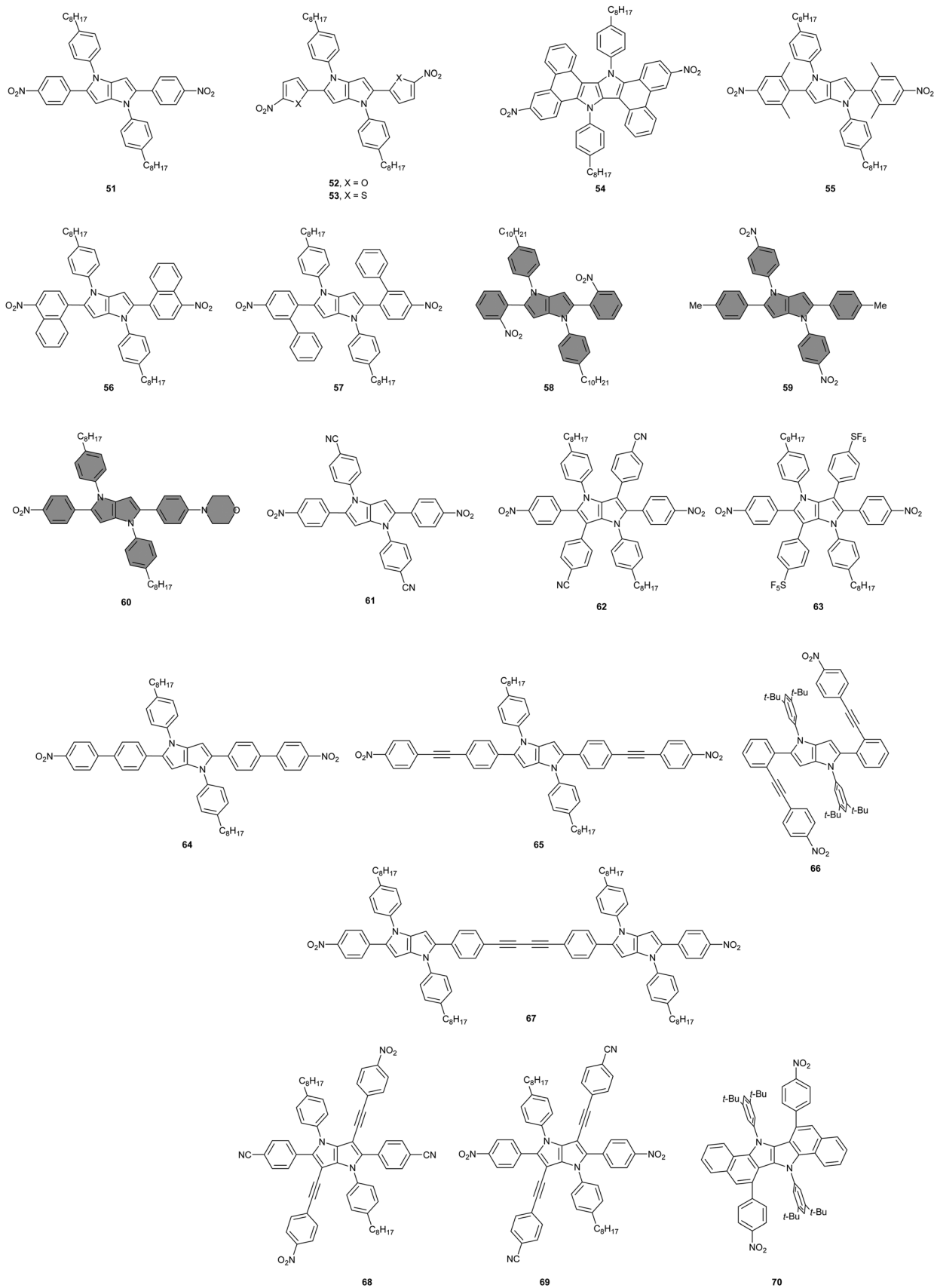
Fig. 22 Structures of tetraaryl-pyrrolopyrroles 51–70 possessing nitro group(s). Fluorescence of dyes colored in gray is below 0.001.
