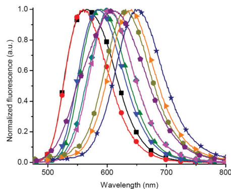
Fig. 21 Normalized fluorescence of 48 in toluene (■), diethyl ether (●), THF (▲), ethyl acetate (▼), \text{CHCl}_3 (◆), \text{CH}_2\text{Cl}_2 (◄), DMF (►), \text{CH}_3\text{CN} (●), DMSO (★) and ethanol (●). Reproduced from ref. 102.
