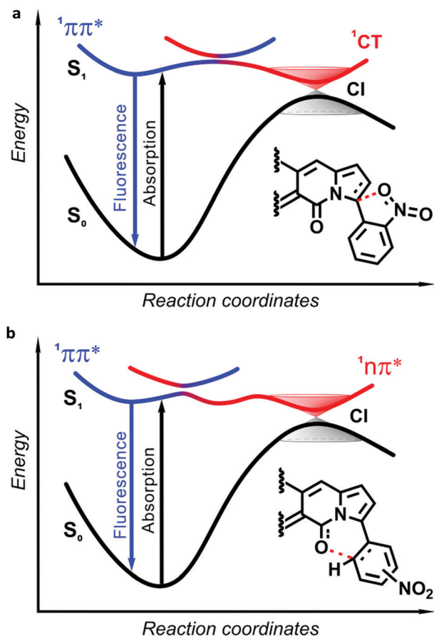
Fig. 30 Schematic diagrams showing the general scenarios of temporal evolution of the photoexcited nitroaryl substituted DPNDs. (a) Excited-state dynamics of ortho -nitrophenyl (and peri -nitronaphthyl) derivatives of DPND. Optical electronic excitation produces locally excited (LE) state with a ^1\pi\pi^* character that adiabatically transitions to a CT twisted state along the S 1 potential-energy trajectory. The photoexcited dyes either deactivate radiatively from ^1\pi\pi^* to S 0 or non-radiatively through ^1\pi\pi^* \rightarrow ^1\text{CT} \rightarrow \text{S}_0 transitions. (b) evolution of photoexcited meta - and para -nitrophenyl substituted DPNDs. Upon photoexcitation, the initially formed fluorescent ^1\pi\pi^* state adiabatically transitions to a twisted non-fluorescent ^1n\pi^* state along the S 1 potential-energy trajectory. The ^1n\pi^* S 1 state forms a CI with the ground state, which accommodates non-radiative deactivation, i.e., ^1\pi\pi^* \rightarrow ^1n\pi^* \rightarrow \text{S}_0 (CI = conical intersection).
