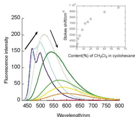
Fig. 7 Fluorescence spectra of 11 in mixed solvents of CH 2 Cl 2 –C 6 H 12 . CH 2 Cl 2 content: 0% (dark blue), 1% (blue), 4% (light blue), 8% (green), 12% (yellowish green), 16% (yellow), 20% (orange), 40% (red) and 60% (dark red). Reproduced from ref. 71.
