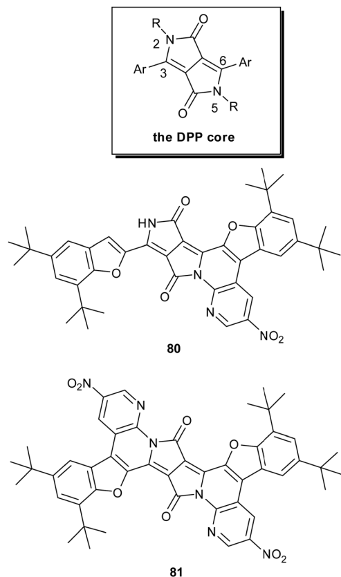
Fig. 26 Structures of dyes 80 and 81 based on the DPP core.
