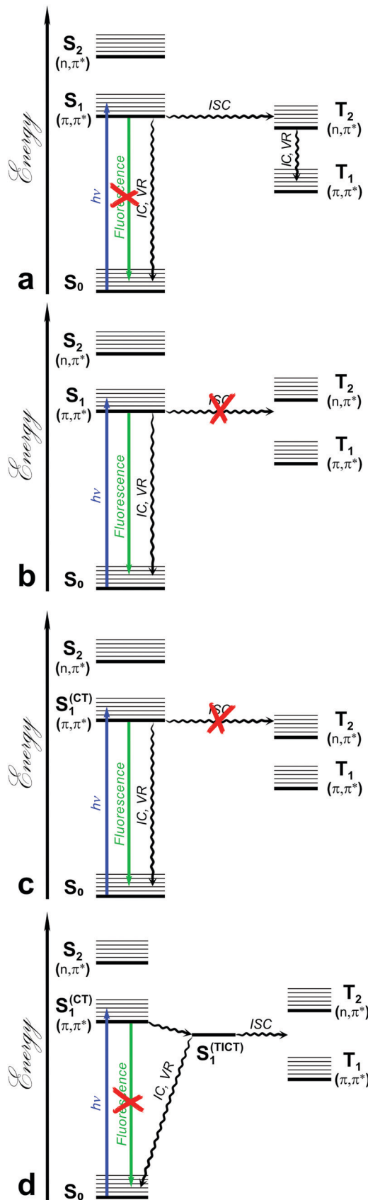
Fig. 34 Jablonski diagrams illustrating possible deactivation pathways of photoexcited nitroaromatic chromophores (ISC = intersystem crossing, IC = internal conversion, and VR = vibrational relaxation).
