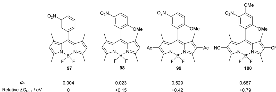
Fig. 32 Structures of 5-(nitrophenyl)BODIPYs 97–100 . Otani and Saito proposed that the same type of quenching mechanism applies to a molecule bearing the pyrrolo[1,2- a ][1,8]naphthylidene chromophore ( 101 ) and a 3-nitroaryl moiety 147 (Fig. 33). This biaryl link between the donor and the acceptor, however, does not guarantee an orthogonal arrangement. Compound 101 is virtually non-luminescent in dichloromethane. According to the authors, protonation at position N-14 increases the reduction potential of the oxidized donor, E_{\text{D}^{\bullet+}/\text{D}}^{(0)} (eqn (5)). That is, this protonation lowers the LUMO level of the pyrrolo[1,2- a ][1,8]naphthylidene chromophore below the LUMO of the nitrophenyl moiety, which inhibits the PET process and allows fluorescence enhancement ( \Phi_f = 0.34 for 101 + \text{H}^+ ). DFT studies confirm almost complete spatial separation of the frontier orbitals within 101 , as the HOMO level is localized over the chromophore, while the LUMO lies exclusively within the 3-nitroaryl moiety. After the protonation event, both, the HOMO and the LUMO are localized predominantly within the principal chromophore core.
