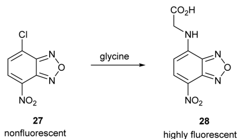
Scheme 1 Transformation of 4-chloro-7-nitrobenzoxadiazole 27 into the fluorescent derivative 28 .
