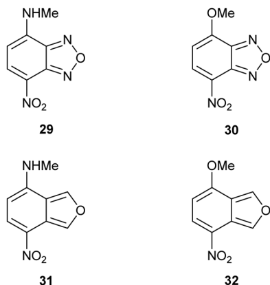
Fig. 16 The structures of nitrobenzo-2-oxa-1,3-diazoles 29 and 30 and the corresponding isobenzofuran derivatives 31 and 32 .
