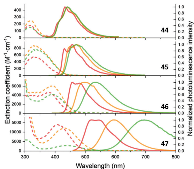
Fig. 19 The absorption (dashed) and the fluorescence (solid) of the phenothiazines 44–47 . Copyright 2020 Wiley. Used with permission from ref. 25.
