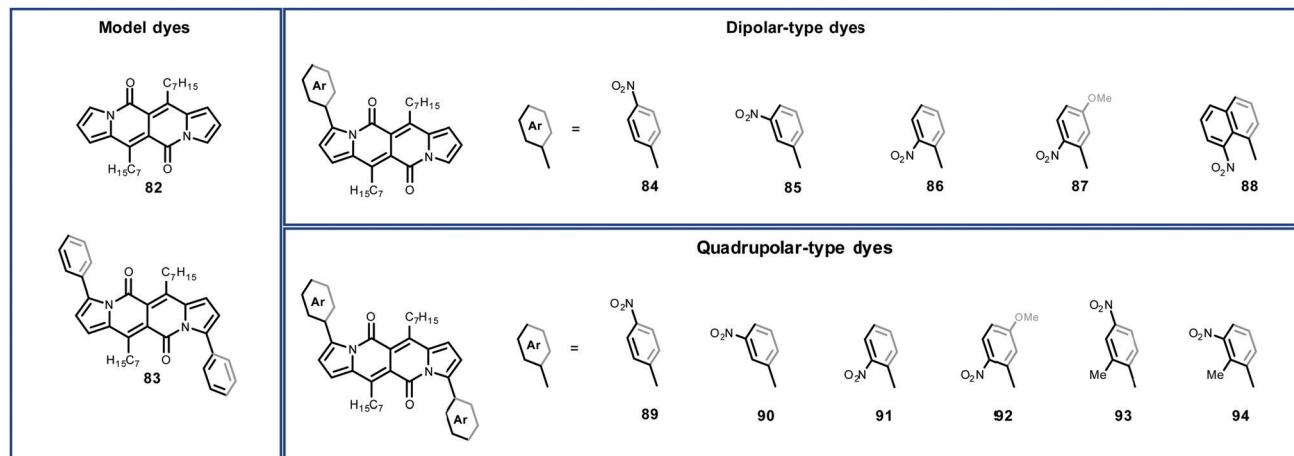
Fig. 29 The structures of bis(nitro)DPNDs 84–94 and parent DPNDs 82 and 83 .
