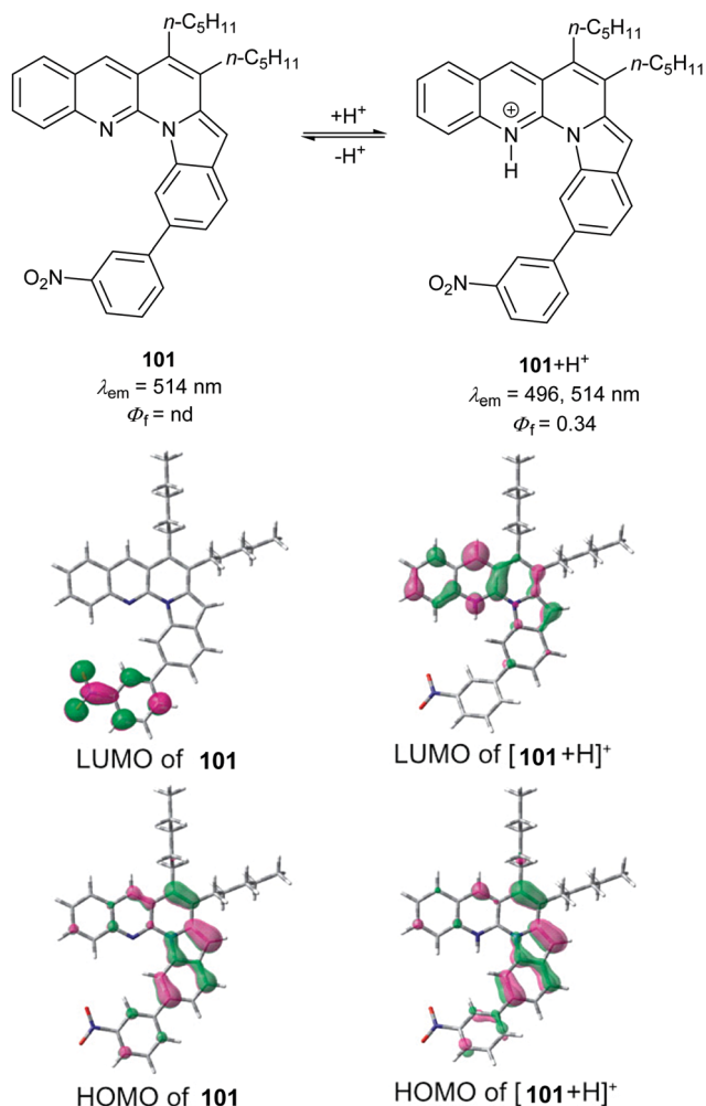
Fig. 33 Chemical structures as well as HOMOs and LUMOs of 101 and its 14-N protonated cation [101 + H] + . nd – not determined. Adapted with permission from ref. 147 Copyright 2014 American Chemical Society.
