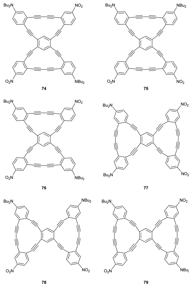
Fig. 25 Structures of nitro-aromatics 74–79 .
