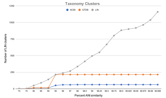
Figure 2: The number of potential taxonomic ranks currently segmenting the Agrobacterium data set. Family, Genus, Species, and Phenotype ranks, when available, were assigned to 70, 80, 95, and 96% ANI similarity respectively.
