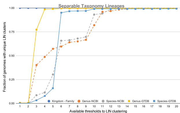
Figure 5: Fraction of genomes that can be uniquely identified using their LIN cluster(s) given how many thresholds can be used for clustering. For both NCBI and GTDB, taxonomy levels Kingdom through Family can all be uniquely identified since our genomes all are part of one Order. The GTDB taxonomic ranks on the Genus and Species levels are more easily separable than the NCBI ranks using the ANI-based LIN clusters.
