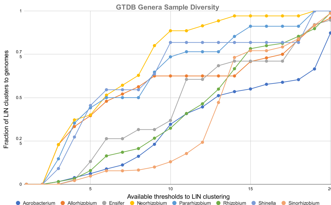
Figure 6: This figure compares all genera in our Agrobacterium data set that have more than ten genomes. The fraction of potential clusters can be taken as a good representative of genome diversity, since higher number of clusters means there exists more separable genomes based on similarity measures, and in extension more genome variation.
