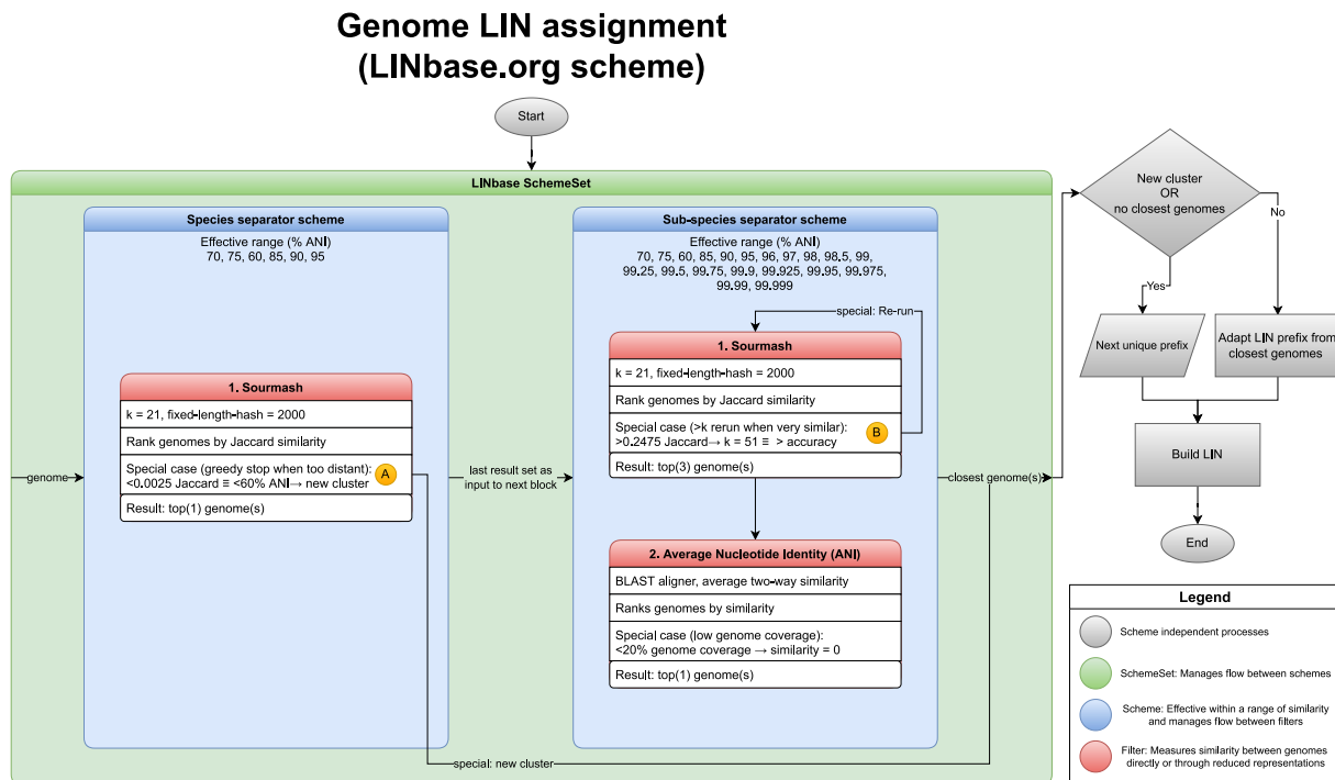
Figure 3: Process of assigning LIN to a single genome sequence using the current LINbase.org LIN scheme. All scheme and measure related criteria can be modified at will to best fit one’s needs.
