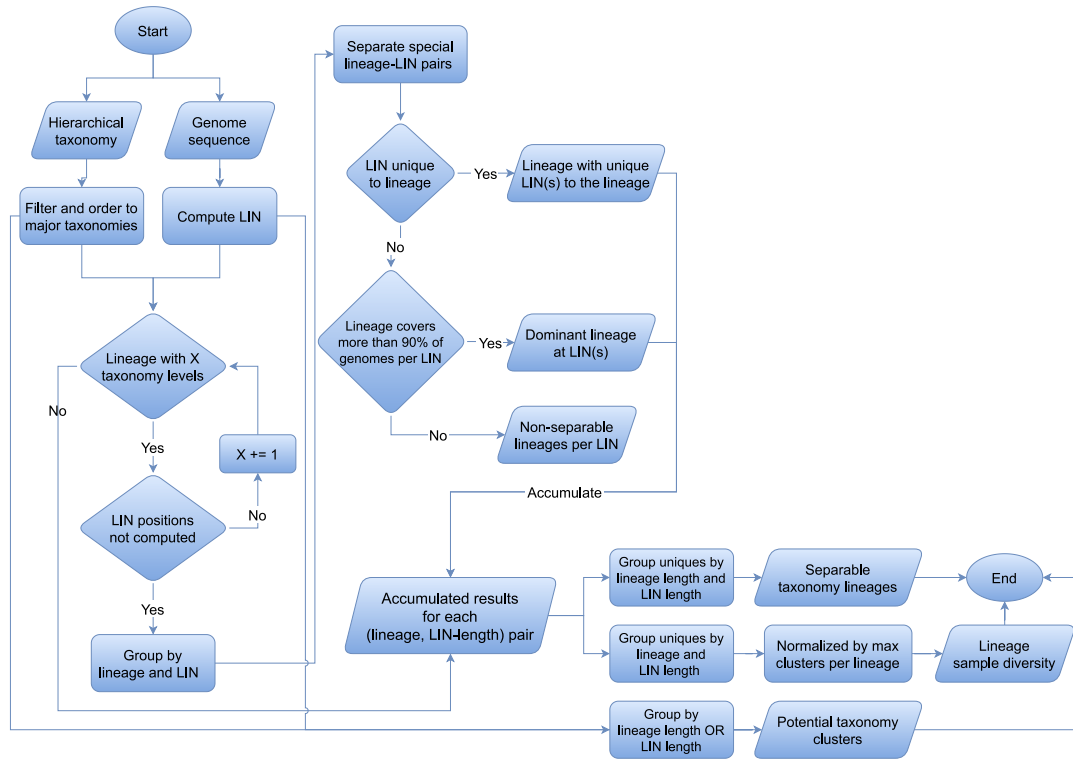
Figure 4: Process of pairing lineage and LIN(s) and how grouping (aggregating) by different parameters results in different views of relation between LIN clusters and the taxonomic lineage. The last three nodes before the end are the three figures included in Section 4.
