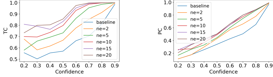
(a) CIFAR-10
