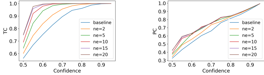
(b) CelebA
