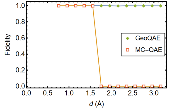
FIG. 3. The fidelity of the ground state of \text{H}_2\text{O} . The H-O-H angle is fixed to the equilibrium angle, \theta = 104.45^\circ . We set T = 40 and M = 20 for both methods.
