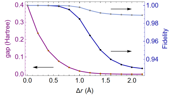
FIG. 17. The dependence of the energy gaps of one-step GeoQAE evolution and the fidelity of the ground-state wave functions of \text{H}_2\text{O} on the bond change \Delta r . The evolution is from H_{\text{full}}^P(r_0) to H_{\text{full}}^P(r_0 + \Delta r) , with initial O-H bond length r_0 = 0.958 \text{ \AA} and H-O-H angle fixed \theta = 104.45^\circ . The gap minimum between the ground state and the first excited state for H(s) = (1-s)H_{\text{full}}^P(r_0) + sH_{\text{full}}^P(r_0 + \Delta r) shows a trend of exponential decay with \Delta r . The upper fidelity curve is obtained with T = 160 and M = 80 and the lower fidelity curve is obtained with T = 40 and M = 20 . There is a substantial improvement using larger T and M values.
