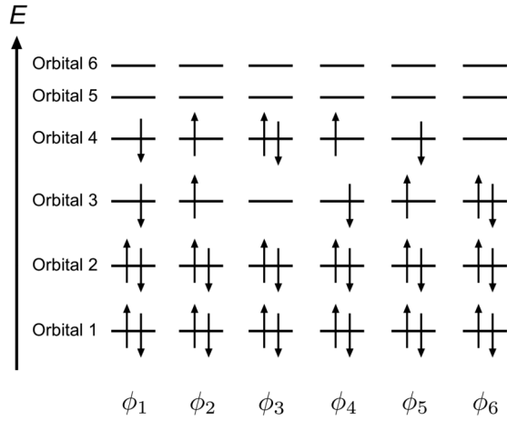
FIG. 4. The spin and orbital configurations for several lowest-energy states of H_i^F(r_0) for \text{CH}_2 near its equilibrium position. The four orbitals are obtained from the Hartree-Fock procedure and the orbital 5 and 6 are empty for all the states we consider here.
