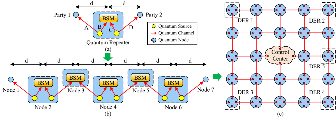
Fig. 8 A QKD-based quantum network using quantum repeaters [31]. (a) Illustration of a quantum repeater. (b) A chain of quantum repeaters. (c) The quantum network. BSM: Bell State Measurement. Quantum node: A quantum repeater (including a node with only the measurement capability) or a communicating party. d : The distance between two quantum nodes.
