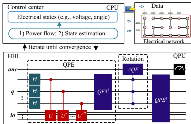
Fig. 2 Quantum circuit architecture for quantum-inspired power grid static analytics
