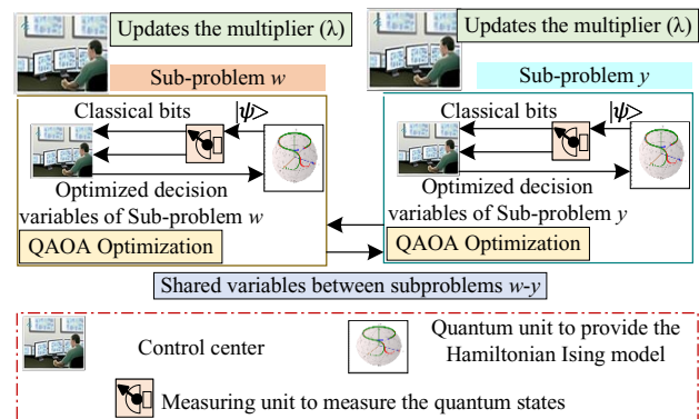
Fig. 5 Schematic of distributed optimization of power systems
