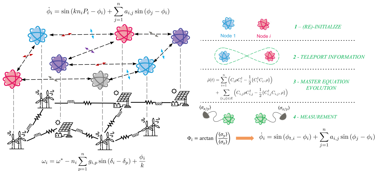
Fig. 7 Coupling of power grids to the network of quantum controllers (left), and schematic depiction of the QDC algorithm (right) [25].
