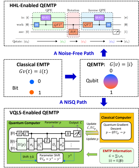
Fig. 3 Schematic of quantum-enabled power system electromagnetic transient analysis
