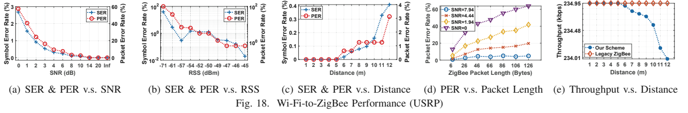
Fig. 18. Wi-Fi-to-ZigBee Performance (USRP)
