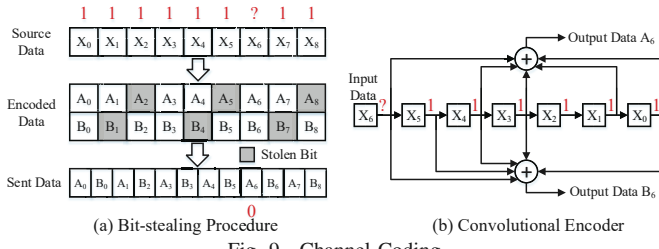
Fig. 9. Channel Coding
