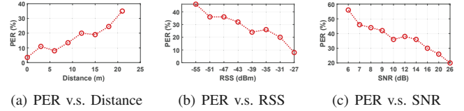
Fig. 19. Wi-Fi-to-ZigBee Performance (COTS Devices)
