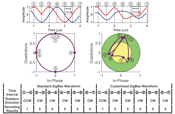
Fig. 11. Comparison of ZigBee Waveform
