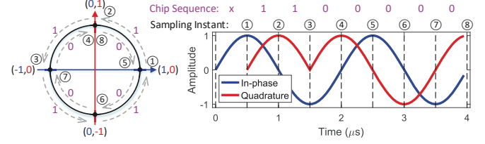
Fig. 2. ZigBee Demodulation Mechanism
