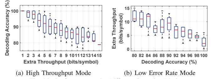
Fig. 15. Performance under Different Operating Modes
