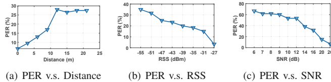
Fig. 21. Wi-Fi-to-Wi-Fi Performance (COTS Devices)
