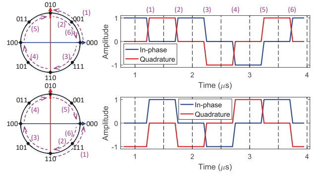
Fig. 6. Principle of Starting Phase Embedding
