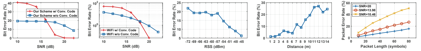
Fig. 20. Wi-Fi-to-Wi-Fi Performance (USRP)
