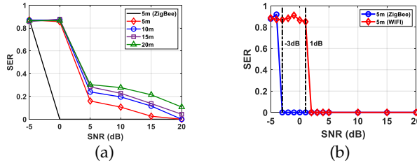
Fig. 21: SER Performance
