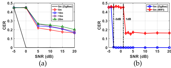
Fig. 20: CER Performance
