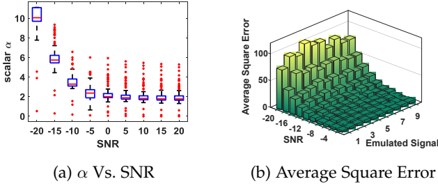
Fig. 15: Quantization Performance
