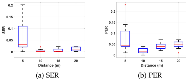
Fig. 13: Signal Emulation Attack on USRP Testbed
