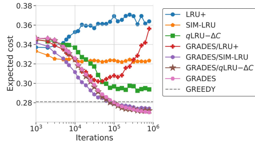
Fig. 4. Expected cost \mathcal{C}(\cdot) incurred by different policies under the trace Synthetic . LRU+, SIM-LRU, q LRU- \Delta C ( q = 10^{-2} ), GREEDY, and GRADES ( \eta = 0.64 , plain and grafted with p = 10^{-1} ). Cache size k = 313 .
