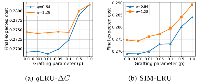
Fig. 5. Effect of the grafting parameter p on the final expected cost \mathcal{C}(\cdot) . GRADES/ q LRU- \Delta C ( q = 10^{-2} ) and GRADES/SIM-LRU for different learning rates under the trace Synthetic . Cache size k = 313 .
