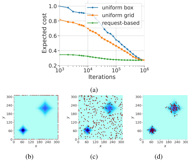
Fig. 6. Subfigure (a) shows the expected cost \mathcal{C}(\cdot) incurred by GRADES/ q\text{LRU}-\Delta C ( \eta = 0.64 grafted with p = 1 and q = 10^{-3} ) for different initialization (uniform box, uniform grid, and request-based depicted in (b), (c), and (d), respectively) under the trace Synthetic . Cache size is k = 313 . The heatmap depicts the popularity distribution of objects in the grid.
