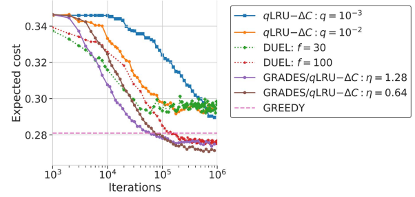
Fig. 8. Expected cost \mathcal{C}(\cdot) incurred by the different policies under the trace Synthetic : q\text{LRU}-\Delta C ( q = 10^{-3}, 10^{-2} ), DUEL, GREEDY, and GRADES ( \eta = 1.28, 0.64 grafted with p = 1 and q = 10^{-3} ). Cache size k = 313 .
