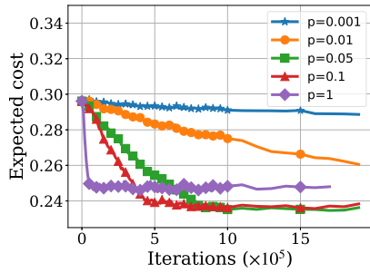
Fig. 7. Effect of grafting parameter p on the expected cost \mathcal{C}(\cdot) in a dynamic setting for GRADES/ q\text{LRU}-\Delta C ( \eta = 0.64 ). The cache is initialized to a stationary configuration as in Fig. 3. Now, only requests corresponding to region B from the trace Synthetic are made. Cache size k = 313 .
