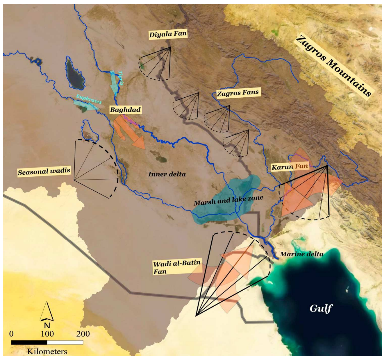
Figure 9. Features of the Tigris-Euphrates-Karun Delta. Black shading represents Tigris-Euphrates-Karun river catchment. Orange arrows represent directional influence of alluvial fan systems on the Mesopotamian Delta's hydrography. Modified from [63,99].
