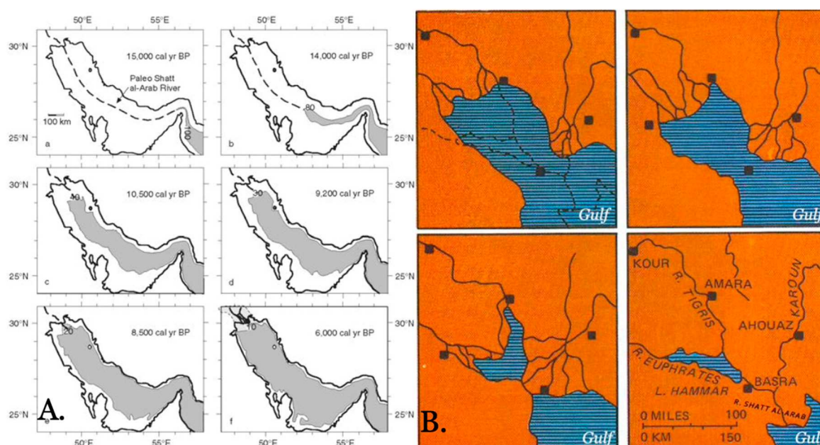
Figure 8. (A) Progression of marine water into the Gulf basin from the Pleistocene to the early Holocene, including the position of a precursor to the Shatt al-Arab that once emptied directly into today's Gulf of Oman (modified from [59]). For scale, see Figure 7. (B) From left to right and top to bottom, hypothetical geomorphodynamics of the formation of the modern deltaic complex during the Middle-Late Holocene: 5000 BP, 4000 BP, 3000 BP, and 2000 BP (modified from [101]).
