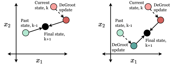
(a) Accelerated averaging model
