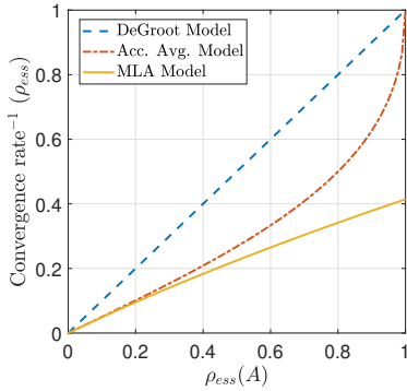
Fig. 3: Comparison of essential spectral radii and the optimal rates of convergence of the three models of network dynamics; DeGroot model, accelerated averaging model, and the MLA model under the criteria given in Theorem 8. MLA model yields faster convergence.
