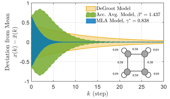
Fig. 4: Comparison of rates of convergence in three averaging models for a ring network with self-loops. The plot shows the envelope enclosed between the maximum and minimum deviation from the mean state and is simulated using 1000 randomly chosen initial conditions. MLA converges faster.
