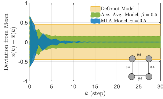
Fig. 2: Comparison of convergence in three averaging models for a periodic network. The plot shows the envelope enclosed between the maximum and minimum deviation from the mean state and is simulated using 1000 randomly chosen initial conditions. In contrast to others, the MLA model converges to consensus.
