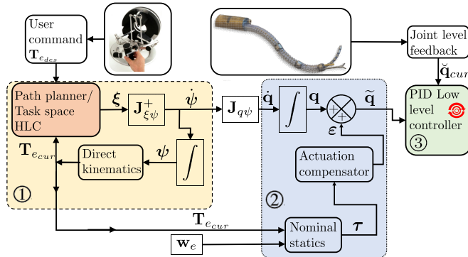
Fig. 9. Position control with a high level controller (HLC) for end-effector motion tracking ①, a feed-forward actuation compensator ②, and a low-level controller (LLC) for joint-level position control ③.
