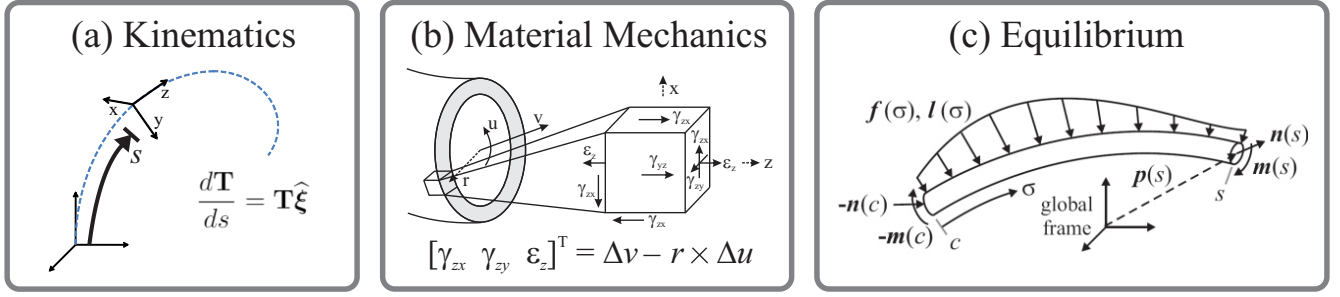
Fig. 6. Continuum robot models are built around three main components: (a) Kinematics relates curvature to the position and orientation along the robot. (b) Constitutive material laws relate stress to strain, linking internal forces to kinematics. (c) Equilibrium equations balance the internal and external loads on the robot. Continuum robot modeling efforts can be categorized based on the choices made in each of these parts.
