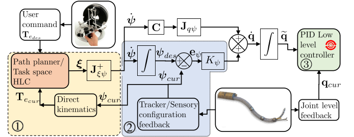
Fig. 10. Position control with mixed configuration and joint space feedback as presented in [165]. Position control with a high level controller (HLC) for end-effector motion tracking ①, a proportional gain configuration space rectifier ②, and a low-level controller (LLC) ③ for joint-level position control.
