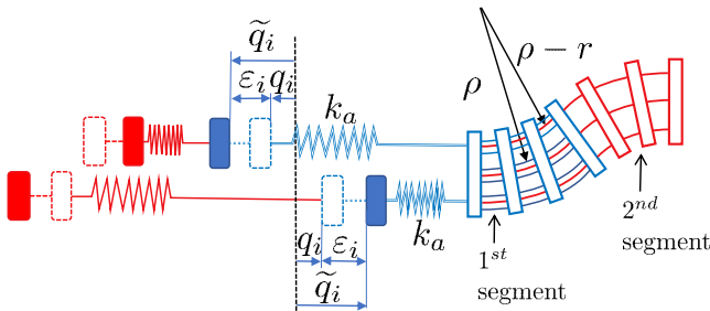
Fig. 7. A two-segment multibackbone continuum robot with concentric backbones. The figure depicts the actuation compensation with one backbone under tension and another under compression for the first segment and the opposite for the second segment. Empty dashed-line rounded-squares designate the nominal joint-level positions q_i and the solid-filled ones show the corrected joint positions \tilde{q}_i with actuation compensation, \epsilon_i . k_a depicts the axial stiffness of the backbones.
