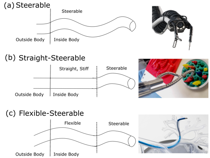
Fig. 2. Continuum robot implementations based on slenderness ratio. (a) Steerable system: entire portion of continuum robot inserted inside body is steerable. Used for slenderness ratios of less than about 50. Example: Medrobotics Flex robot with steerable sheath [30]. (b) Straight-steerable system: robot is comprised of a straight stiff proximal section with a steerable distal section for slenderness ratios of about 100. Example: Titan Medical Enos single-port robot with straight-steerable arms [14]. (c) Continuum robot is comprised of a passive flexible proximal section and a steerable distal section for slenderness ratios of 100 to over 1500. Example: Auris Heath Monarch robotic endoscope [28]
