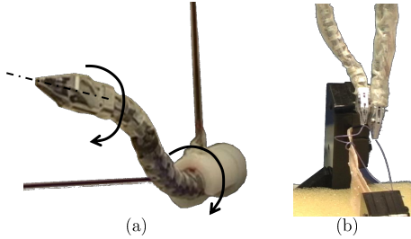
Fig. 8. Rotation transmission along the backbone of a multibackbone robot requires accurate joint-level motion coordination. (a) rotation about the backbone [80], (b) dual arm suturing where the left arm uses rotation about the backbone and the right arm is used for needle hand-off.
