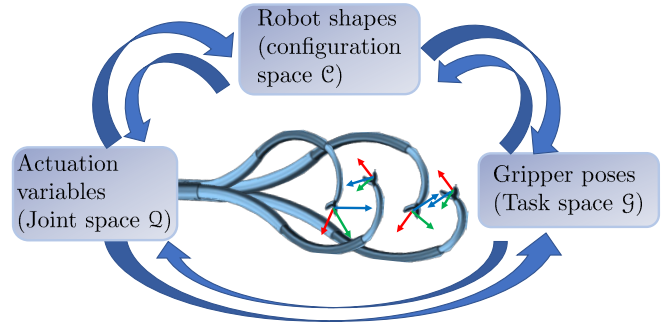
Fig. 5. Kinematic mappings used for control and modeling.
