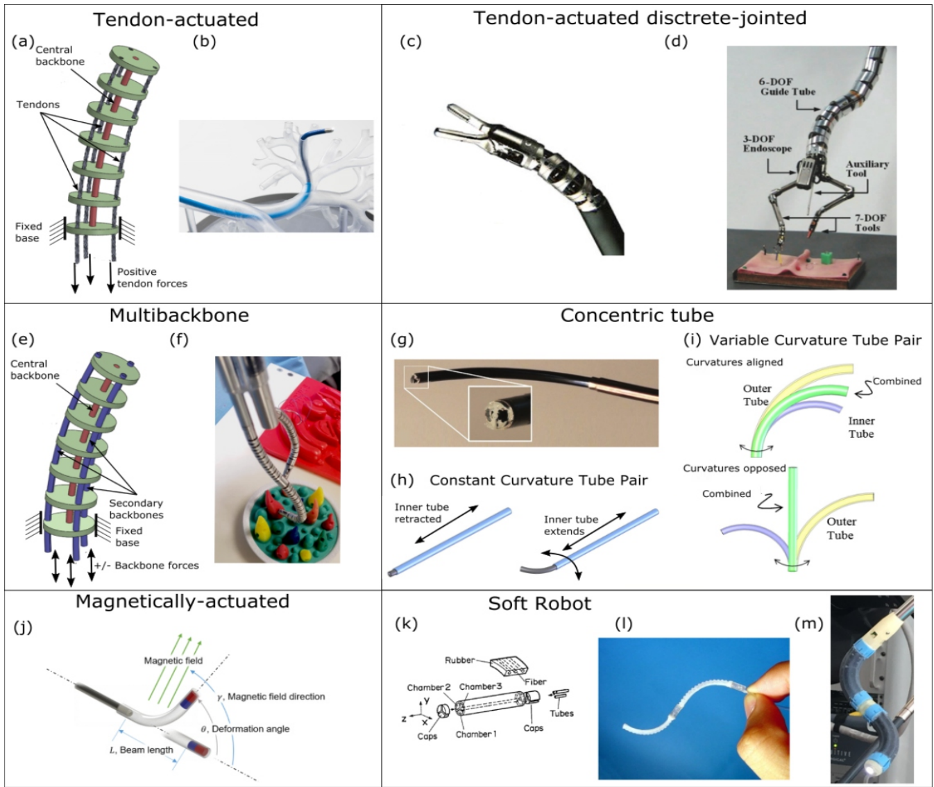
Fig. 1. Continuum robot design classification. (a) In tendon-actuated designs, tendons run through channels in disks attached to central backbone. In many clinical applications, central backbone and disks are replaced by a tube with small lumens for each tendon plus a larger central lumen. (b) Tendon-actuated Auris Health Monarch robotic endoscope. (c) Intuitive Surgical's 5mm diameter laparoscopic instrument [12]. (d) Steerable sheath of Samsung's NOTES robot [13]. (e) Multibackbone actuation replaces the tendons with secondary backbones that can exert both tensile and compressive forces on the structure. (f) Multibackbone arms of Titan Medical Enos single-port robot [14]. (g) Concentric tube robot comprised of telescoping sections of either constant or variable curvature [15]. (h) Constant curvature tube pair is comprised of precurved inner tube that conforms to shape of stiffer outer tube when retracted. (i) Variable curvature tube pair is comprised of tube pair of approximately equal stiffness and precurvature. Relative rotation of the combined tubes varies curvature from maximum value to approximately straight. (j) Magnetically-actuated catheter. Magnetic dipole embedded in robot tip experiences a torque causing it to move toward alignment with an externally generated magnetic field (from [10]). (k) Soft robots use pneumatic actuation. Here, sheath is comprised of 3 internal chambers that can be independently pressurized. Acting as tensile tendons, the pressurized chambers cause the robot to bend (from [16]). (l) Soft multi-segment catheter (from [17]). (m) Stiff-flop soft medical robot [18].
