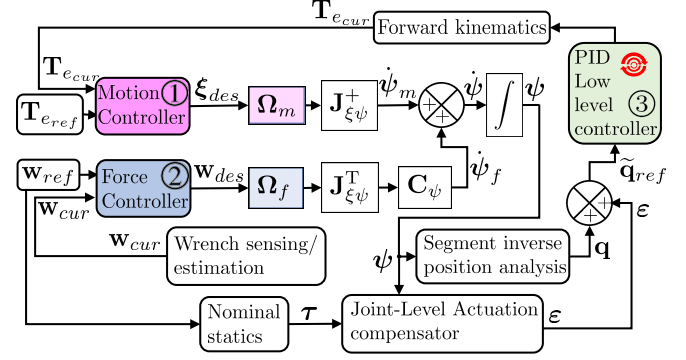
Fig. 11. Hybrid motion/force control for continuum robots. A motion controller ① and a force controller ② act in decoupled spaces yielding configuration space speeds that are integrated to produce joint-level reference input to a low-level controller ③ after implementing actuation compensation.
