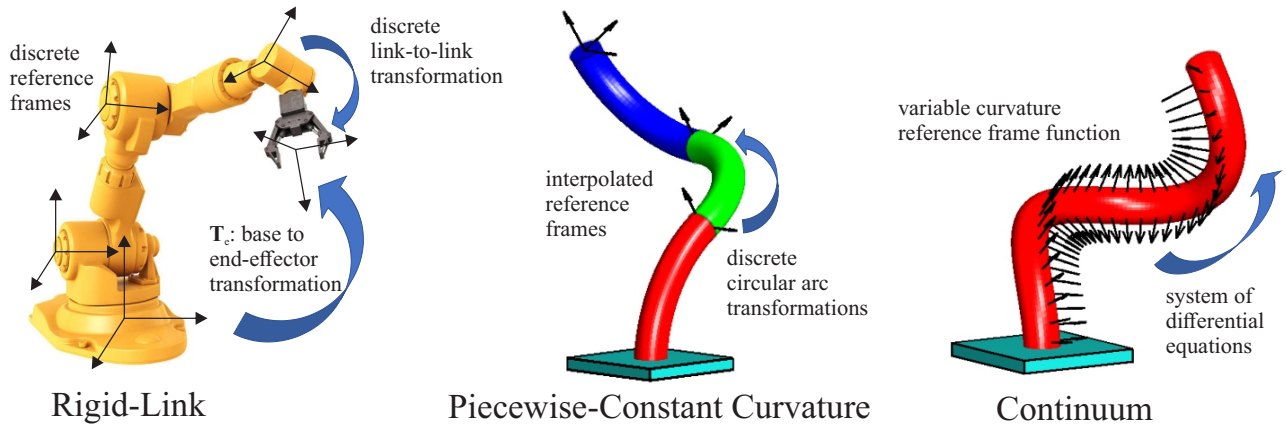
Fig. 4. Continuum robot kinematics models differ from conventional rigid-link models in that they must capture bending along the entire length, rather than at discrete joints only. (a) Rigid link robot with kinematics computed using coordinate frames attached to each robot link. End-effector coordinate frame is related to base coordinate frame by transformation, \mathbf{T}_e(\mathbf{q}) . (b) Simplified robot models use geometric assumption that robot shape consists of piecewise-constant curvature circular arcs. (c) More general robot models account for variable curvature deformations, material mechanics, and external loads. The shape is the solution to a set of differential equations.
