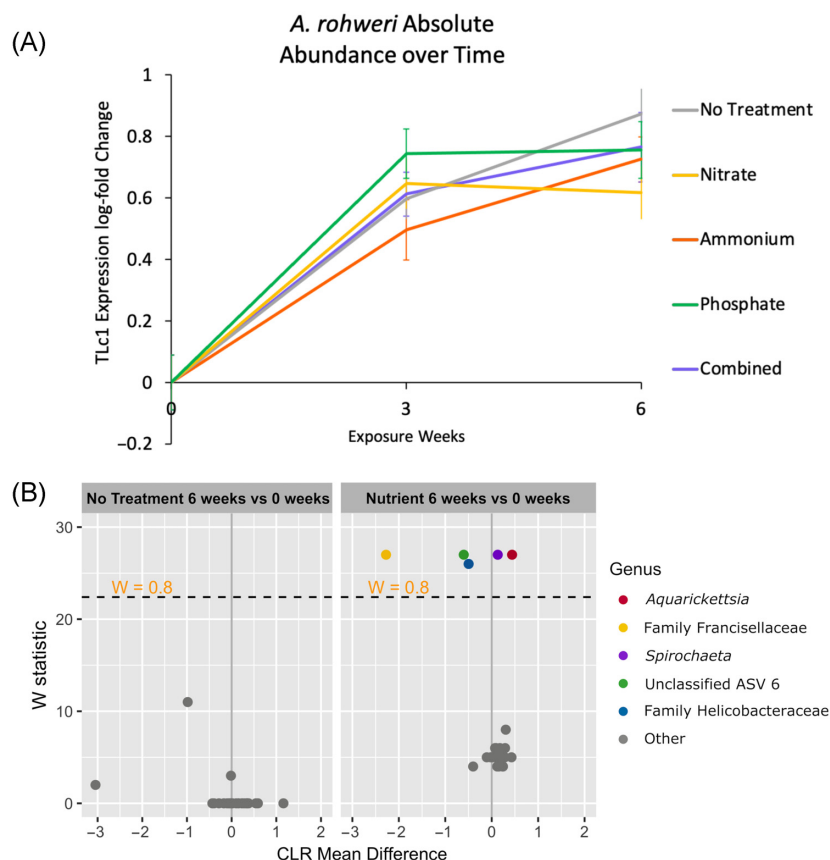
Figure 3. (A). Log-transformed absolute abundance of A. rohweri as determined by quantitative PCR. Samples exposed to high and low concentrations of each nutrient were pooled for analysis. The average log-transformed RQ of all timepoint zero samples ( n = 62 ) was subtracted from log-transformed RQ of samples at weeks 3 and 6 to assess change in absolute abundance over time. (B). Volcano plot of results from differential abundance analysis with ANCOM-II. Analysis performed on genus-level ASV table was filtered to include taxa with a total count of 10 in at least 20% of samples ( n_{\text{taxa}} = 29 ) was used. ANCOM tests the null-hypothesis that the average abundance of a given species in a group is equal to that in the other group. Contrasts were performed within full ASV table subset to either only no treatment samples, or all other treatments pooled together. The W statistic represents the strength of the test for the 29 tested species and is the number of times the null-hypothesis was rejected for a given species. Taxa above the dashed line are significant with the null-hypothesis rejected 80% of the time ( W = 0.8 ). Nonsignificant taxa in any contrast are colored grey. The x-axis value presents the effect size as the CLR-transformed mean difference in abundance of a given species between the two groups being compared. For the second panel, a positive x-axis value means the genus was more abundant at 6 weeks of nutrient treatment compared to 0 weeks or vice versa for a negative x-axis value.
