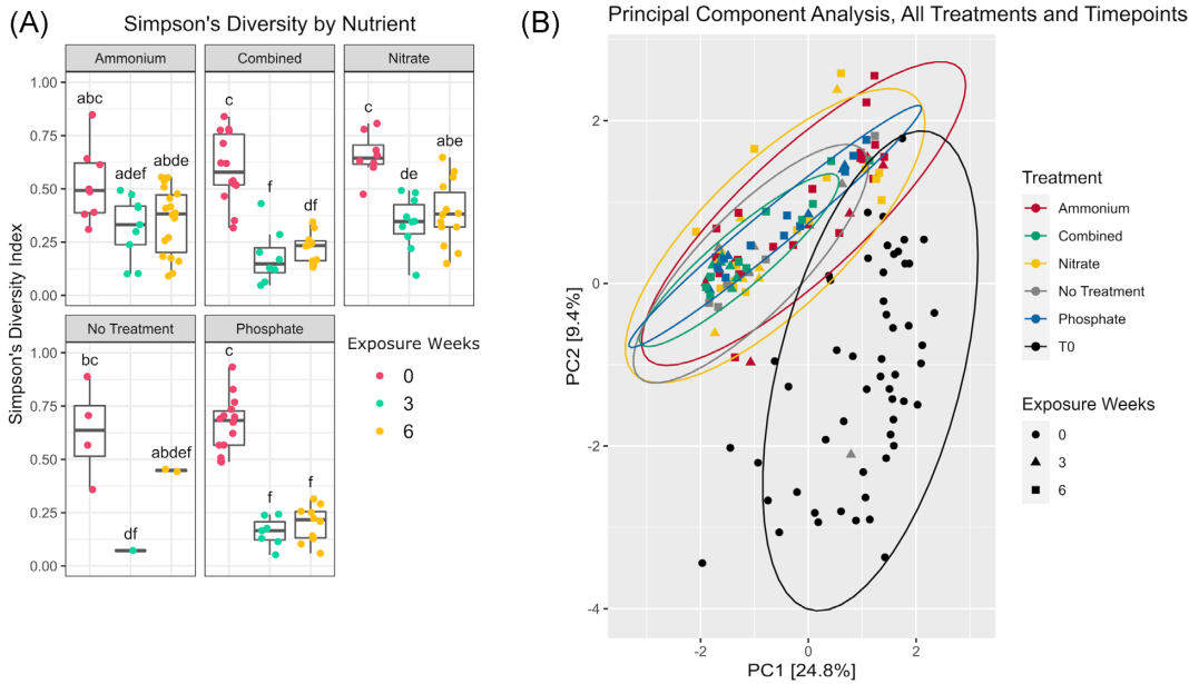
Figure 2. Community diversity metrics by treatment (Ammonium, Combined, Nitrate, Phosphate, or no treatment) and exposure weeks (0, 3, and 6). (A) Simpson's diversity index. Boxes sharing a letter are not significantly different from each other using an FDR corrected significance level of P < .05 . (B) PCA ordination of samples using Euclidean distance on CLR-transformed data.
