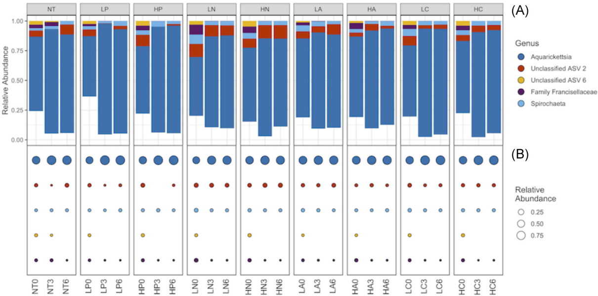
Figure 1. Mean relative abundance of the most abundant genera across three time points in coral fragments exposed to different nutrient constituents. (A) Barplot, showing dominance of Aquarickettsia across all samples. Taxa are included in the plot if they had a relative abundance greater than 1% across the entire dataset. Each bar represents a minimum of three replicates. (B) Bubble plot, showing changes in top five taxa across treatment groups and timepoints. NT = no treatment, L = low (3x ambient), H = high (4x ambient), P = phosphate, N = nitrate, A = ammonium, and C = combined (P, N, and A).
