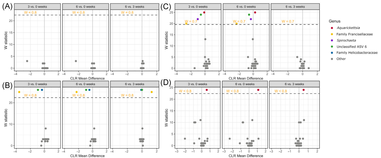
Figure 4. Volcano plots of results from differential abundance analysis with ANCOM-II by individual nutrient treatment. (A). Ammonium (B). Nitrate (C). Combined (D). Phosphate. Analysis performed on genus-level ASV table was filtered to include taxa with a total count of 10 in at least 20% of samples ( n_{\text{taxa}} = 29 ) was used. ANCOM tests the null-hypothesis that the average abundance of a given species in a group is equal to that in the other group. Contrasts were performed as subsets of each individual treatment from full ASV table. The W statistic represents the strength of the test for the 29 tested species and is the number of times the null-hypothesis was rejected for a given species. Taxa above the dashed line are significant with the null-hypothesis rejected 80% of the time ( W = 0.8 ), or 70% of the time for combined treatment samples ( W = 0.7 ). Nonsignificant taxa in any contrast are colored grey. The x-axis value presents the effect size as the CLR-transformed mean difference in abundance of a given species between the two groups being compared.
