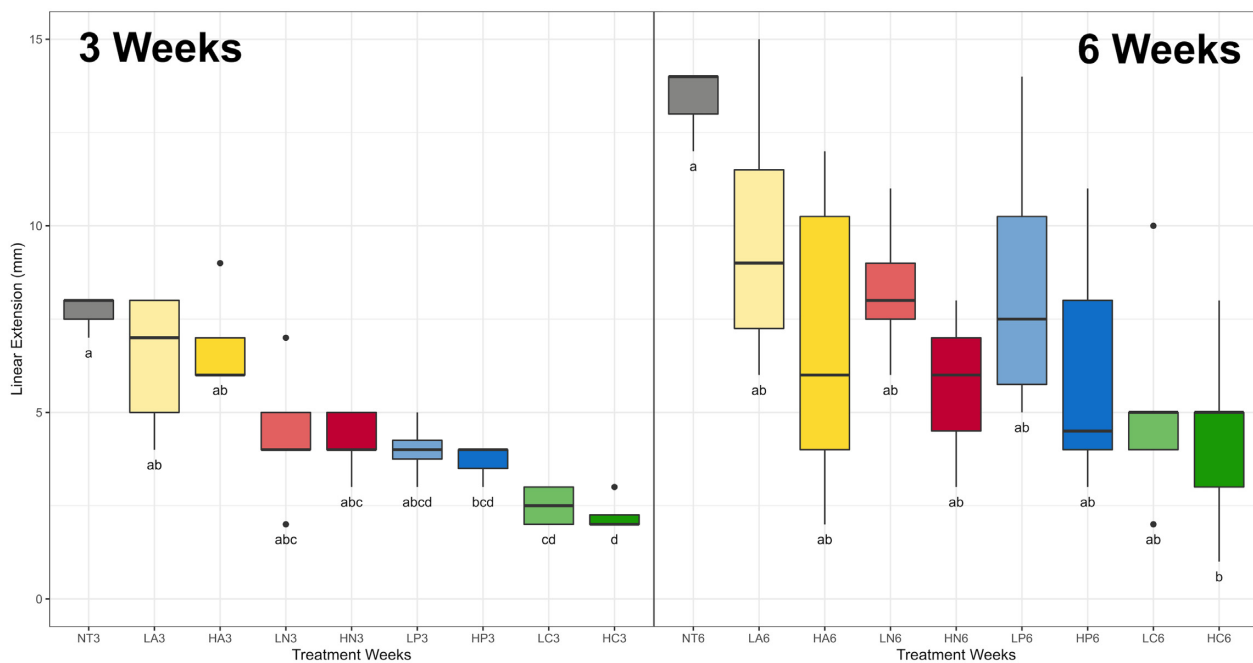
Figure 5. TLE calculated from measurements taken at 0, 3, and 6 weeks of nutrient exposure. Tukey's honest significance test was used on log-transformed data to identify significant differences in mean TLE by nutrient treatment and exposure weeks. Untransformed data is plotted for clarity. Boxes sharing a letter are not significantly different from each other using a significance level of P < .05 .
