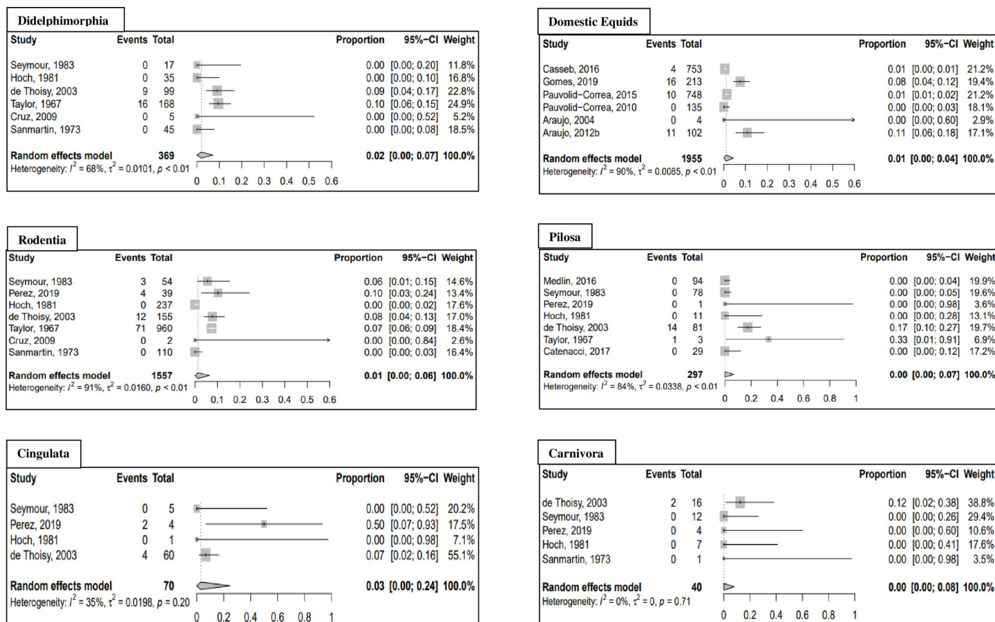
Fig 4. Forest plots of mammal orders (excluding primates) from meta-analysis of pooled MAYV seroprevalence. Estimates are based on random effects model with Freeman-Tukey double arcsine transformation. All samples that tested MAYV-positive are included, regardless of test method.
