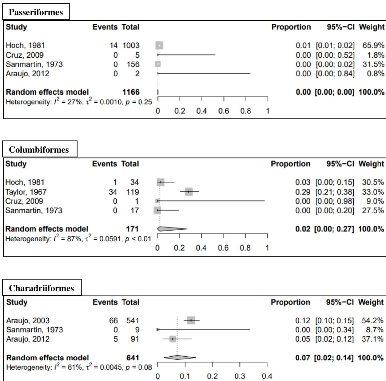
Fig 5. Forest plots of avian orders from meta-analysis of pooled MAYV seroprevalence. Estimates are based on random effects model with Freeman-Tukey double arcsine transformation. All samples that tested MAYV-positive are included, regardless of test method.
