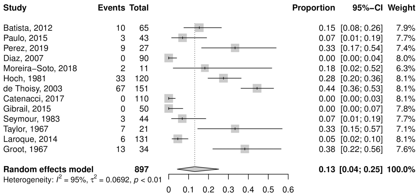
Fig 3. Forest plot of non-human primates from meta-analysis of pooled MAYV seroprevalence. Estimates are based on random effects model with Freeman-Tukey double arcsine transformation. All samples that tested MAYV-positive are included, regardless of test method.
