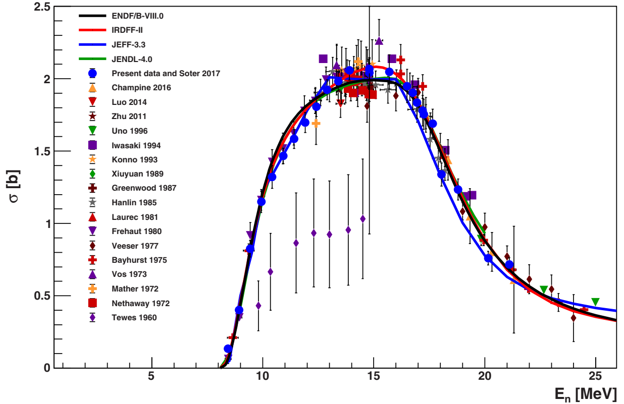
FIG. 2. The present measurements of the ^{169}\text{Tm}(n, 2n)^{168}\text{Tm} cross section compared to previous measurements and evaluations. Only measurements spanning multiple neutron energies are shown.
