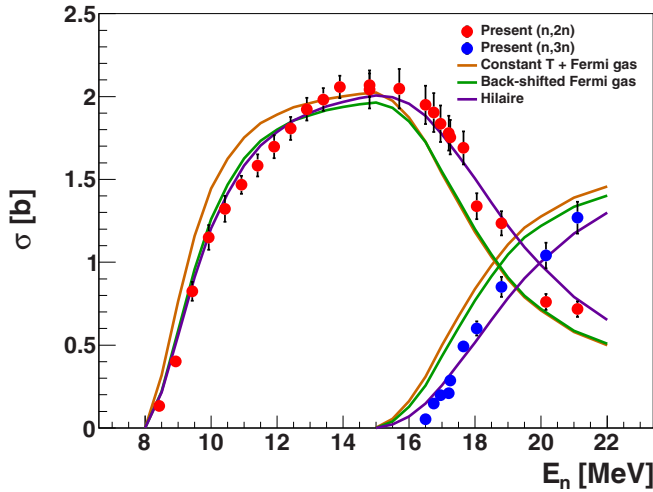
FIG. 4. The present measurements of the ^{169}\text{Tm}(n, 2n)^{168}\text{Tm} and ^{169}\text{Tm}(n, 3n)^{167}\text{Tm} cross sections compared to different TALYS models. See text for a discussion of the models.
