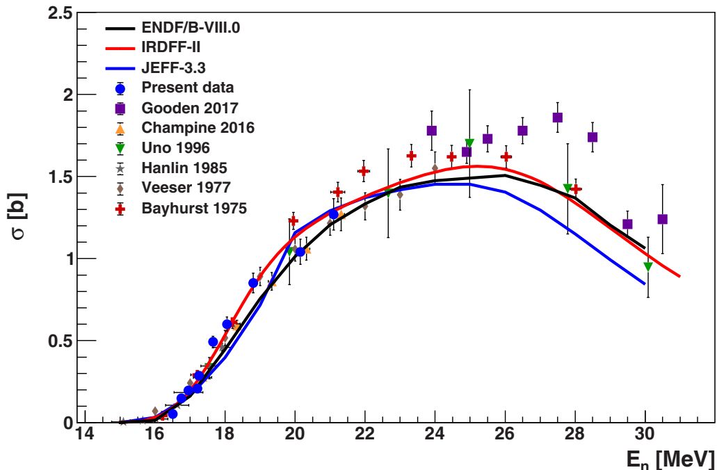
FIG. 3. The present measurements of the ^{169}\text{Tm}(n, 3n)^{167}\text{Tm} cross section compared to previous measurements and evaluations.
