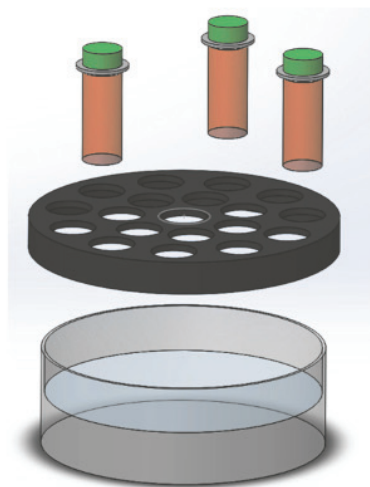
Figure A1. A computer-aided design (CAD) representation of the apparatus used to control temperature during degradation studies of PLA.
