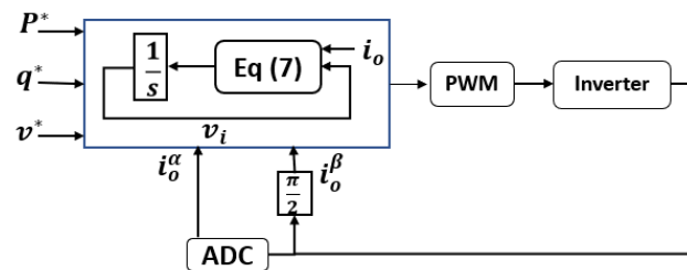
Figure 14. Control architecture of dVOC.
