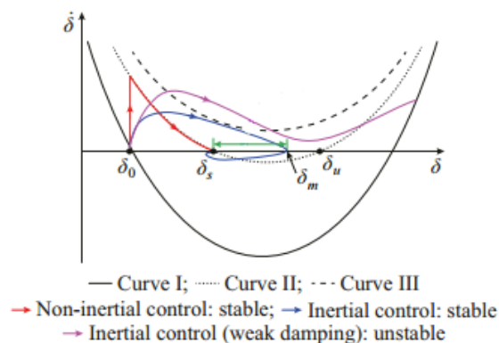
Figure 5. Phase portrait of GFM control [50].
