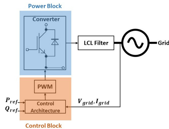
Figure 10. Synchronverter.
