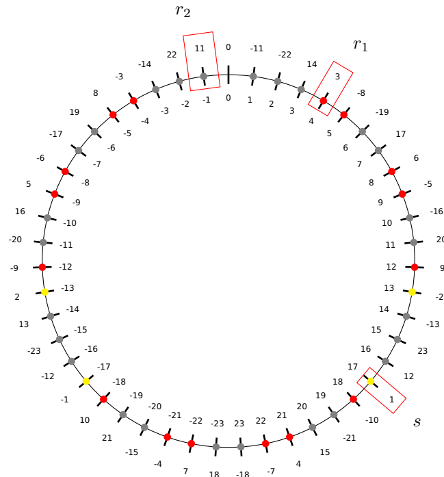
Figure 1: We visualize \mathbb{Z}/47\mathbb{Z} , whose elements are labeled inside the circles. With s = 17 , we label [\cdot]_s for each element on the outside of the circle. Following the positive s -steps, we can see that r_1 is the first time that the path has visited (-s/2, s/2) , at which time the path turn from yellow to red. Similarly, at the 11^{th} s -step, we visit -1 and it is the first time we visit the interval (-r_1/2, r_1/2) .
