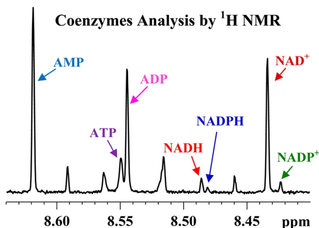
FIGURE 4 Expanded spectral region from an 800 MHz ^1\text{H} NMR spectrum of a mouse liver tissue extract obtained using a 5 mm sample tube showing the characteristic fingerprint of the redox and energy coenzymes. Figure reprinted with permission from Nagana Gowda GA, Abell L, Lee CF, Tian R, Raftery D. Simultaneous analysis of major coenzymes of cellular redox reactions and energy using ex vivo ^1\text{H} NMR spectroscopy. Analytical Chemistry 2016;88(9):4817-4824. Copyright 2016 American Chemical Society
