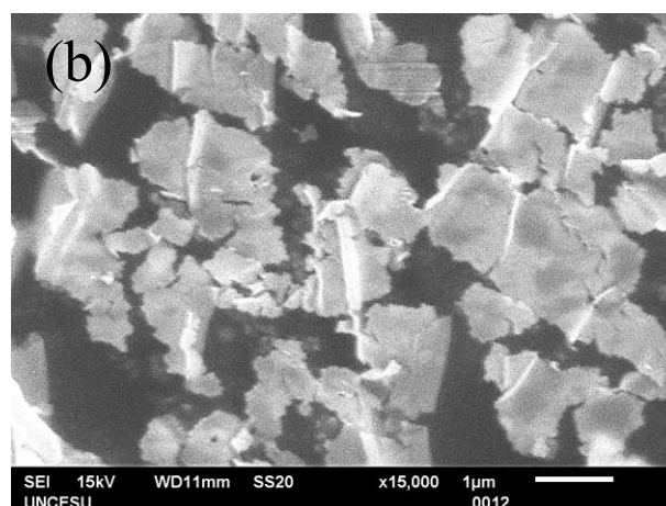
Figure 2. SEM images of exfoliated KLTO perovskite oxide powders at a low magnification (a) and high magnification (b).
