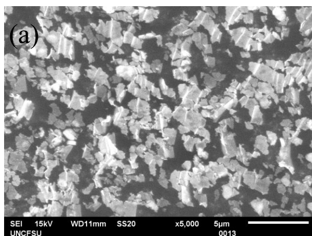
Figure 2. SEM images of exfoliated KLTO perovskite oxide powders at a low magnification (a) and high magnification (b).
