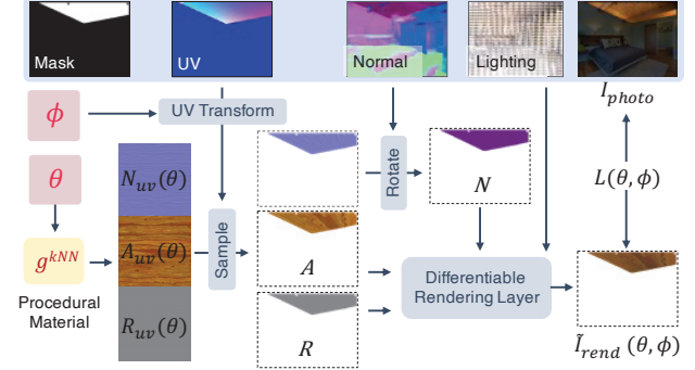
Figure 5. Given a material part mask, UV, scene normals and lighting (top), we construct a fully differentiable pipeline from material graph ( \theta ) and UV transformation ( \phi ) parameters via a texture-to-image mapping and differentiable rendering layer to a rendered image. We optimize for these parameters by comparing this rendering to the input photo.
